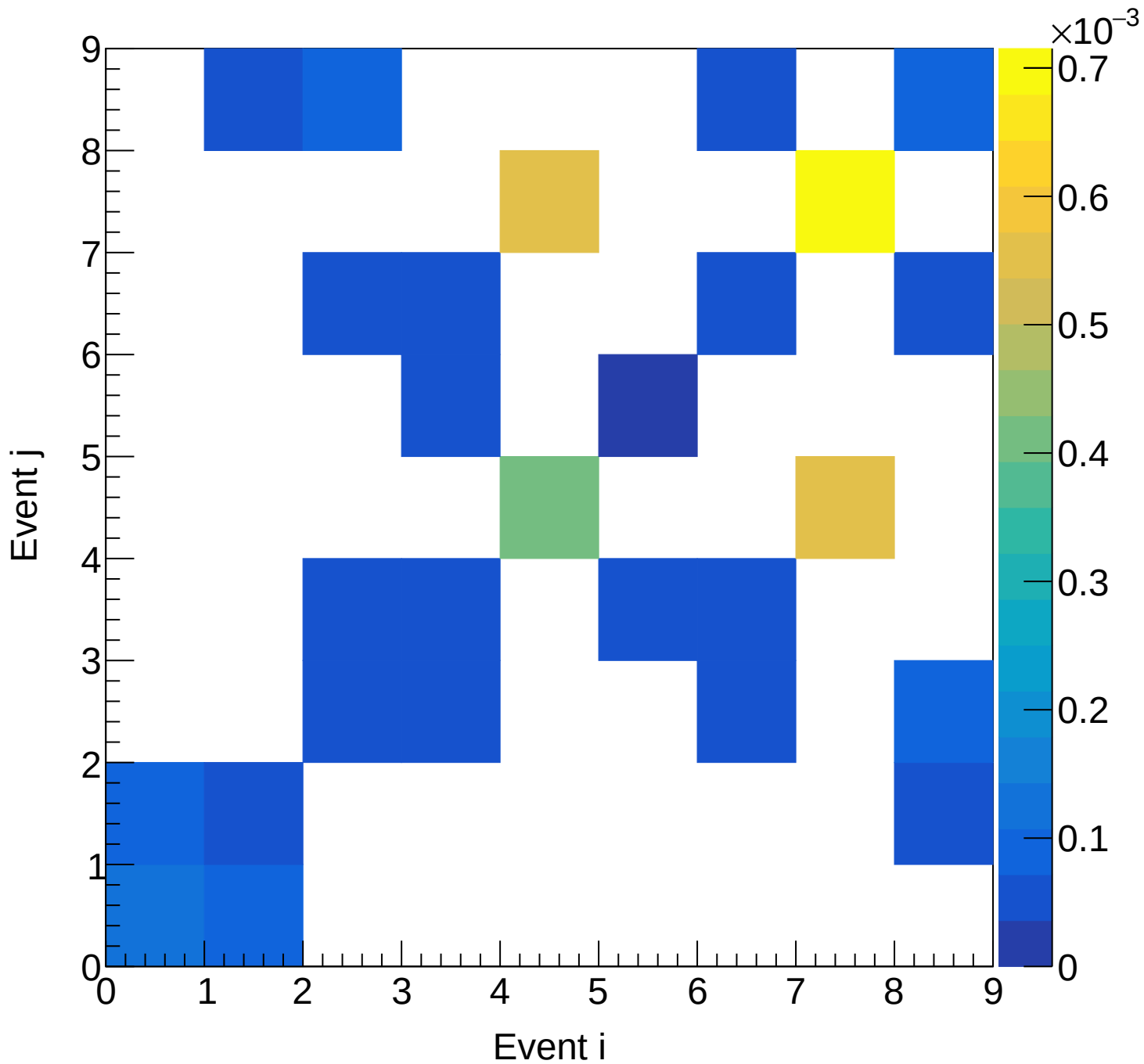
LD2 (total) Covariance | M: [6.6, 6.9] xF: [0.65, 0.70)
