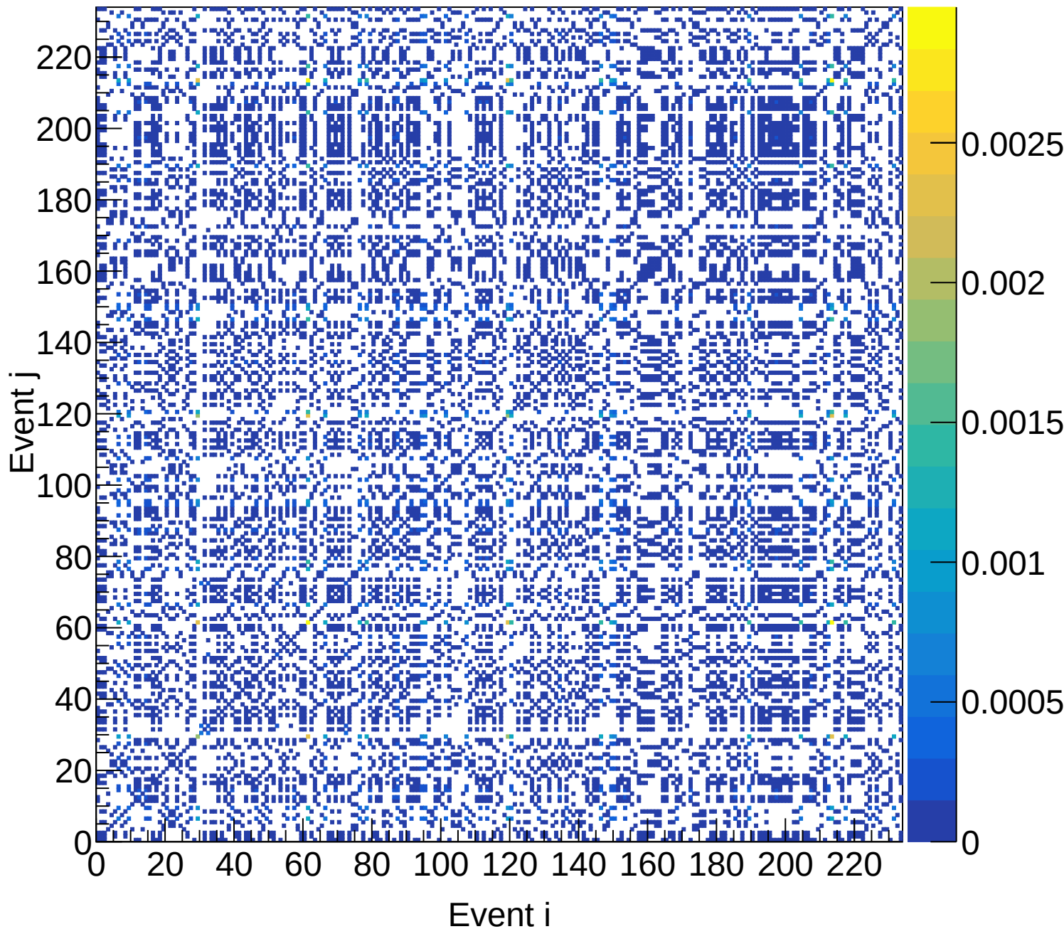
LD2 (total) Covariance | M: [3.9, 4.2) xF: [0.70, 0.75)
