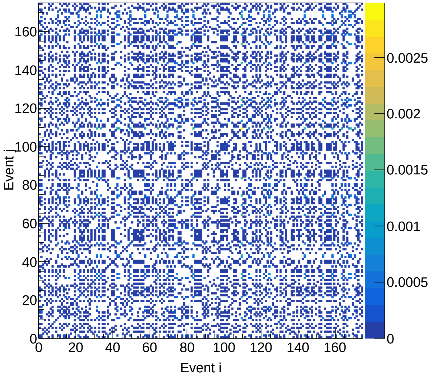
LD2 (total) Covariance | M: [4.2, 4.5) xF: [0.70, 0.75)
