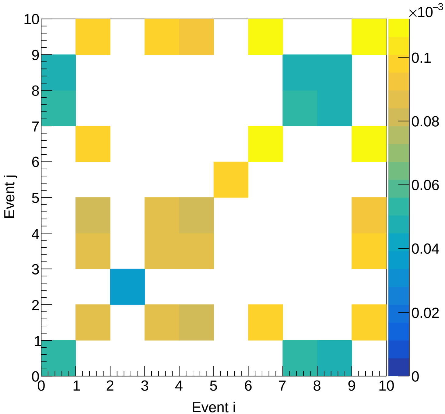
LD2 (total) Covariance | M: [6.0, 6.3) xF: [0.70, 0.75)
