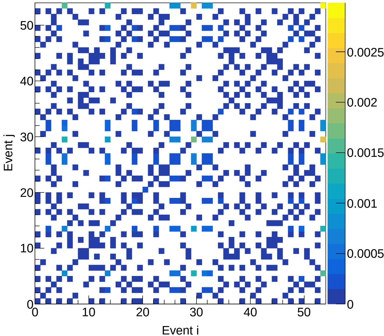
LD2 (total) Covariance | M: [5.4, 5.7) xF: [0.00, 0.05)
