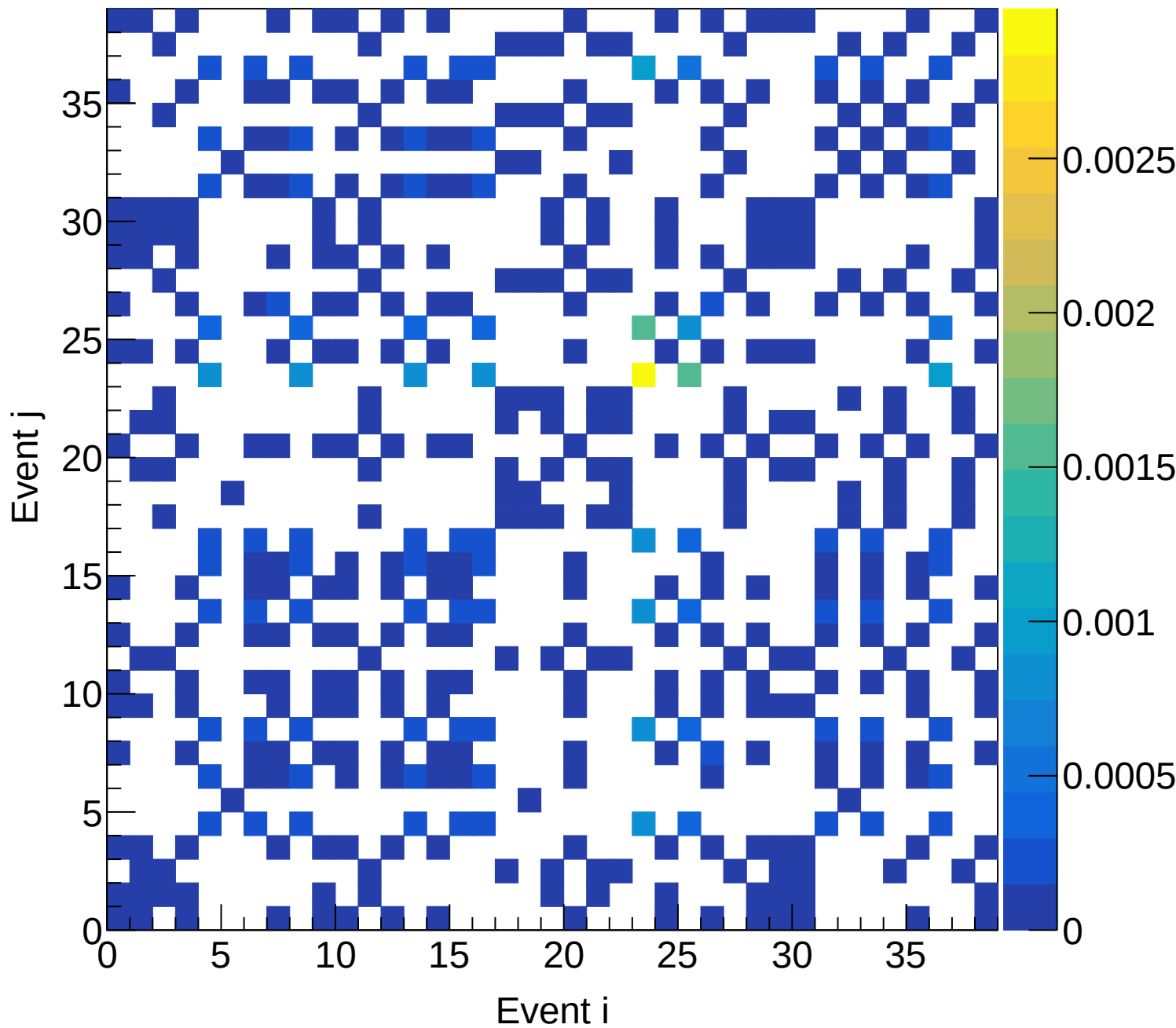
LD2 (total) Covariance | M: [5.7, 6.0] xF: [0.00, 0.05)
