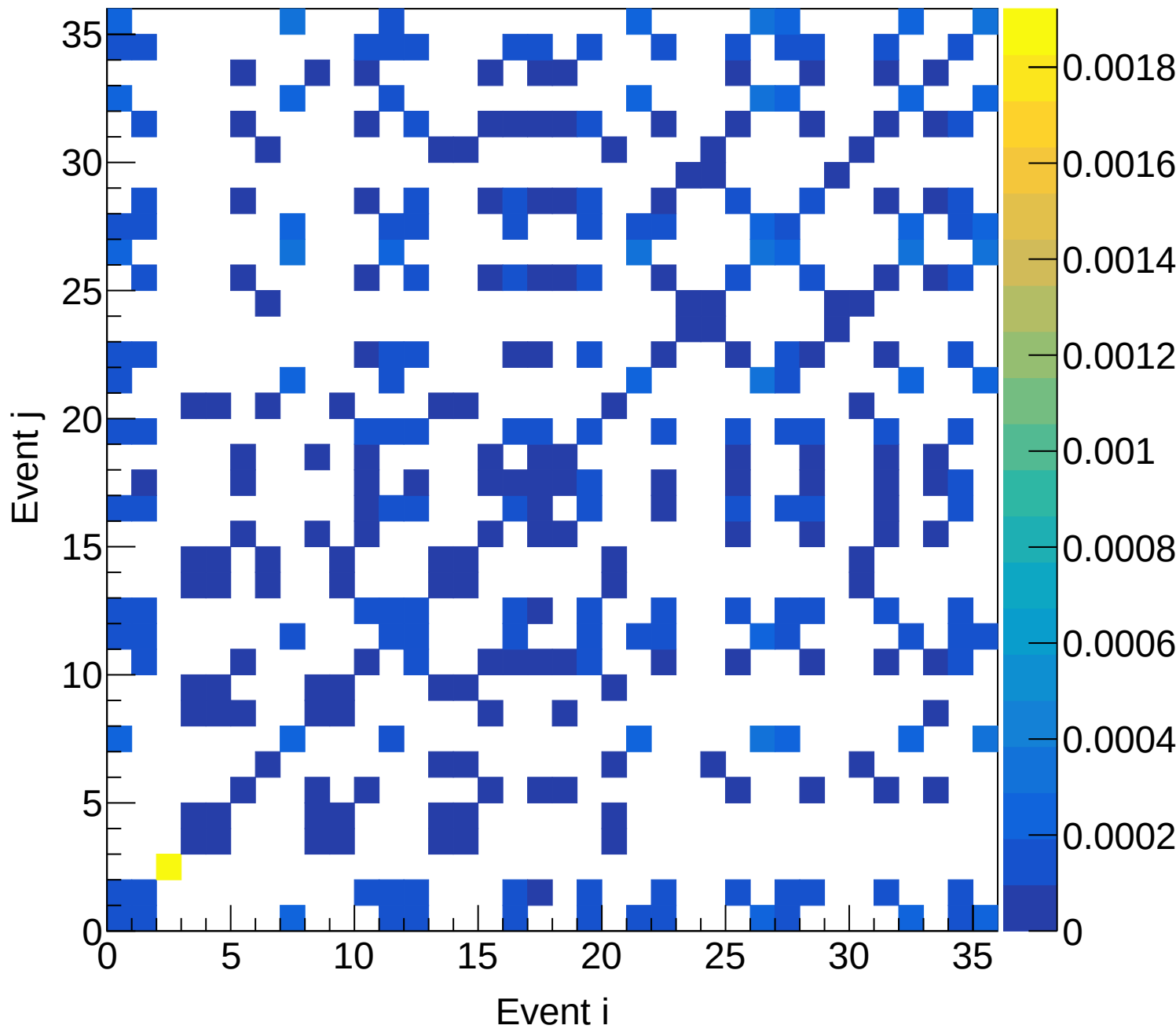
LD2 (total) Covariance | M: [6.0, 6.3] xF: [0.00, 0.05]
