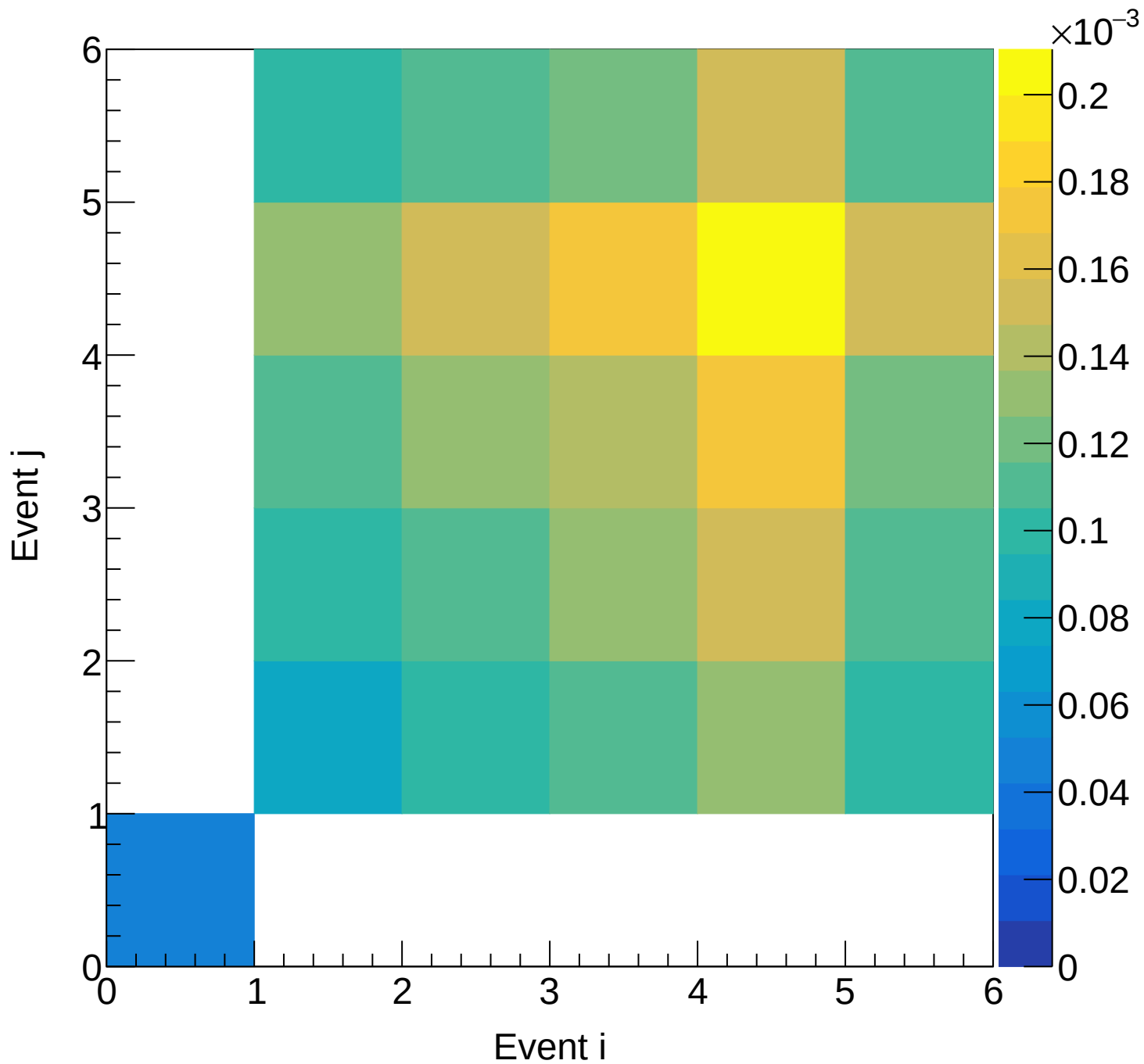
LD2 (total) Covariance | M: [6.6, 6.9) xF: [0.00, 0.05)
