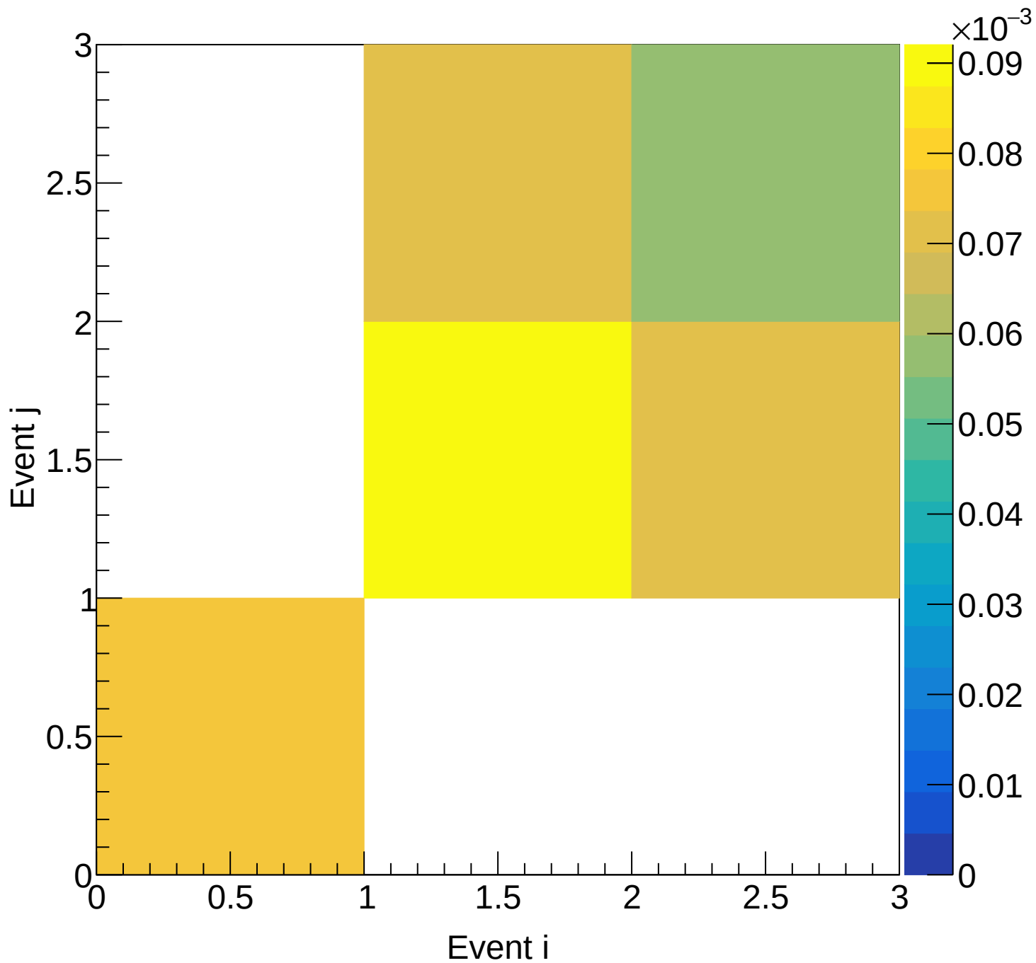
LD2 (total) Covariance | M: [4.2, 4.5) xF: [0.05, 0.10)
