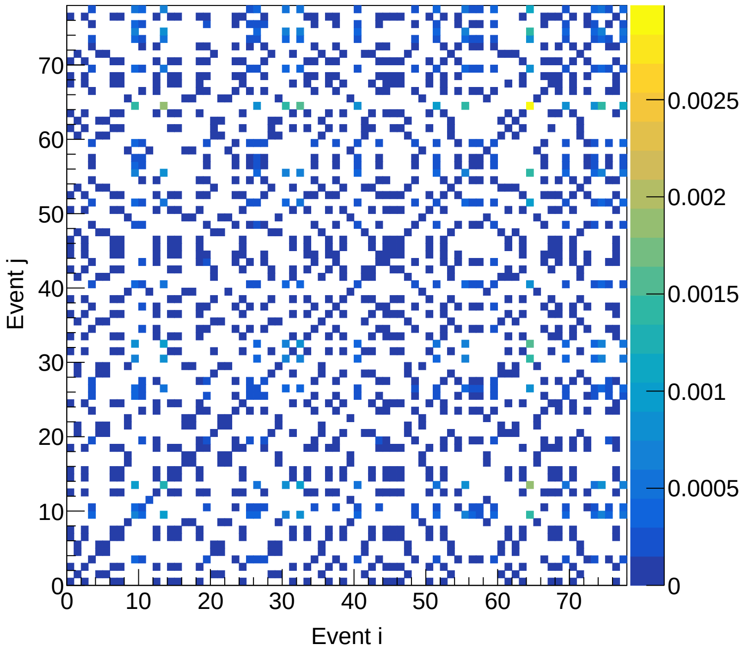
LD2 (total) Covariance | M: [5.7, 6.0) xF: [0.05, 0.10)
