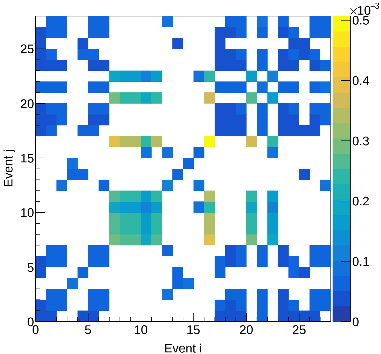
LD2 (total) Covariance | M: [6.3, 6.6) xF: [0.05, 0.10)
