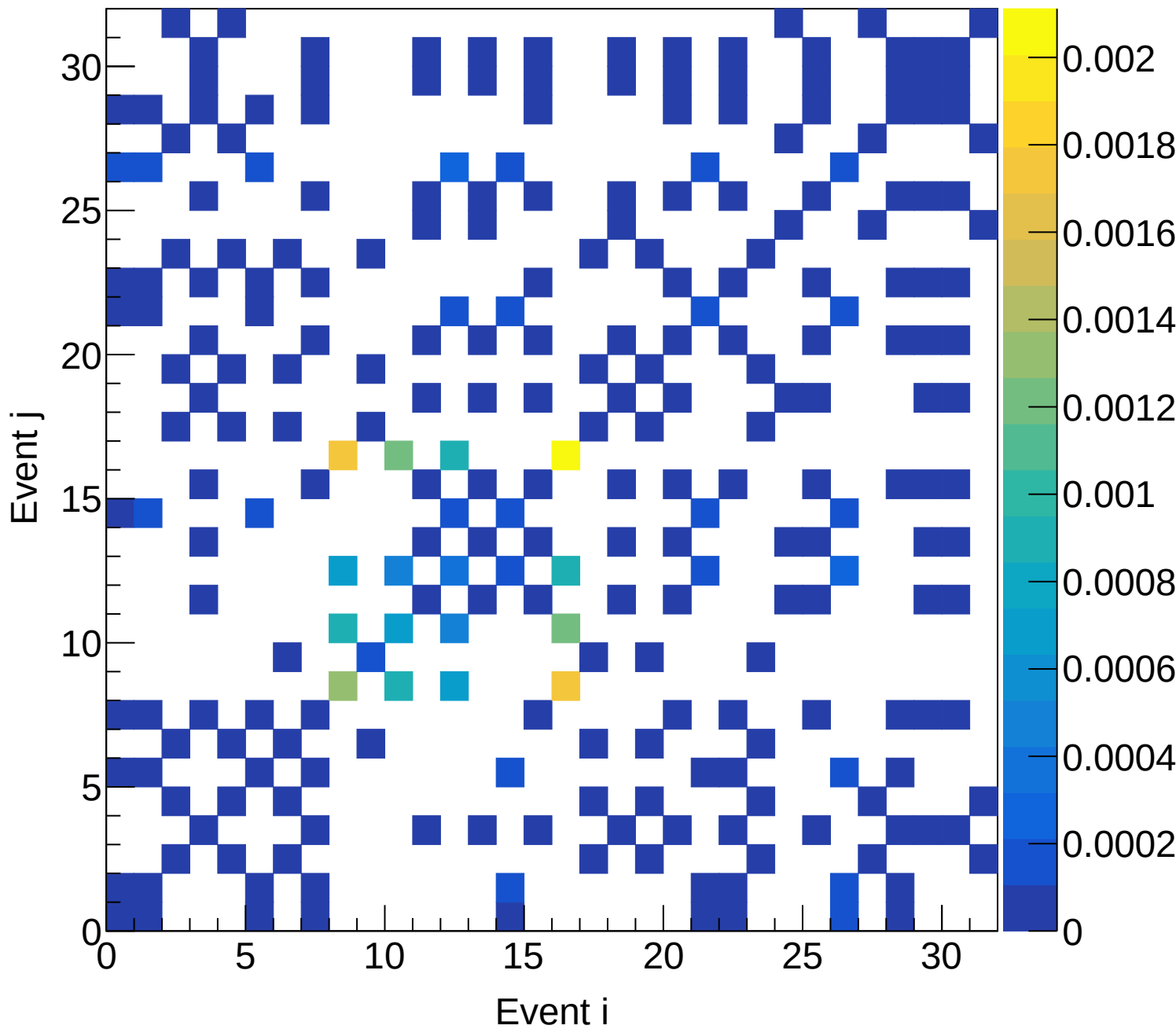
LD2 (total) Covariance | M: [4.2, 4.5) xF: [0.10, 0.15)
