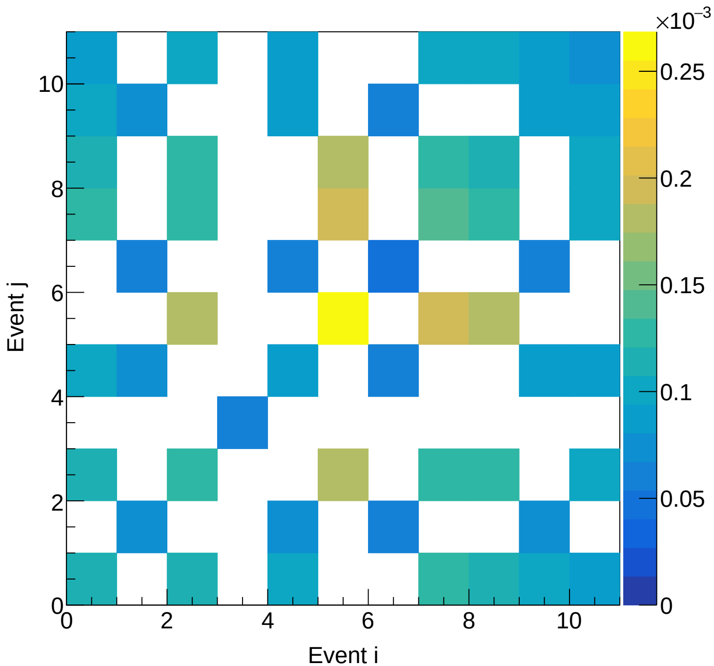
LD2 (total) Covariance | M: [6.9, 7.5) xF: [0.10, 0.15)
