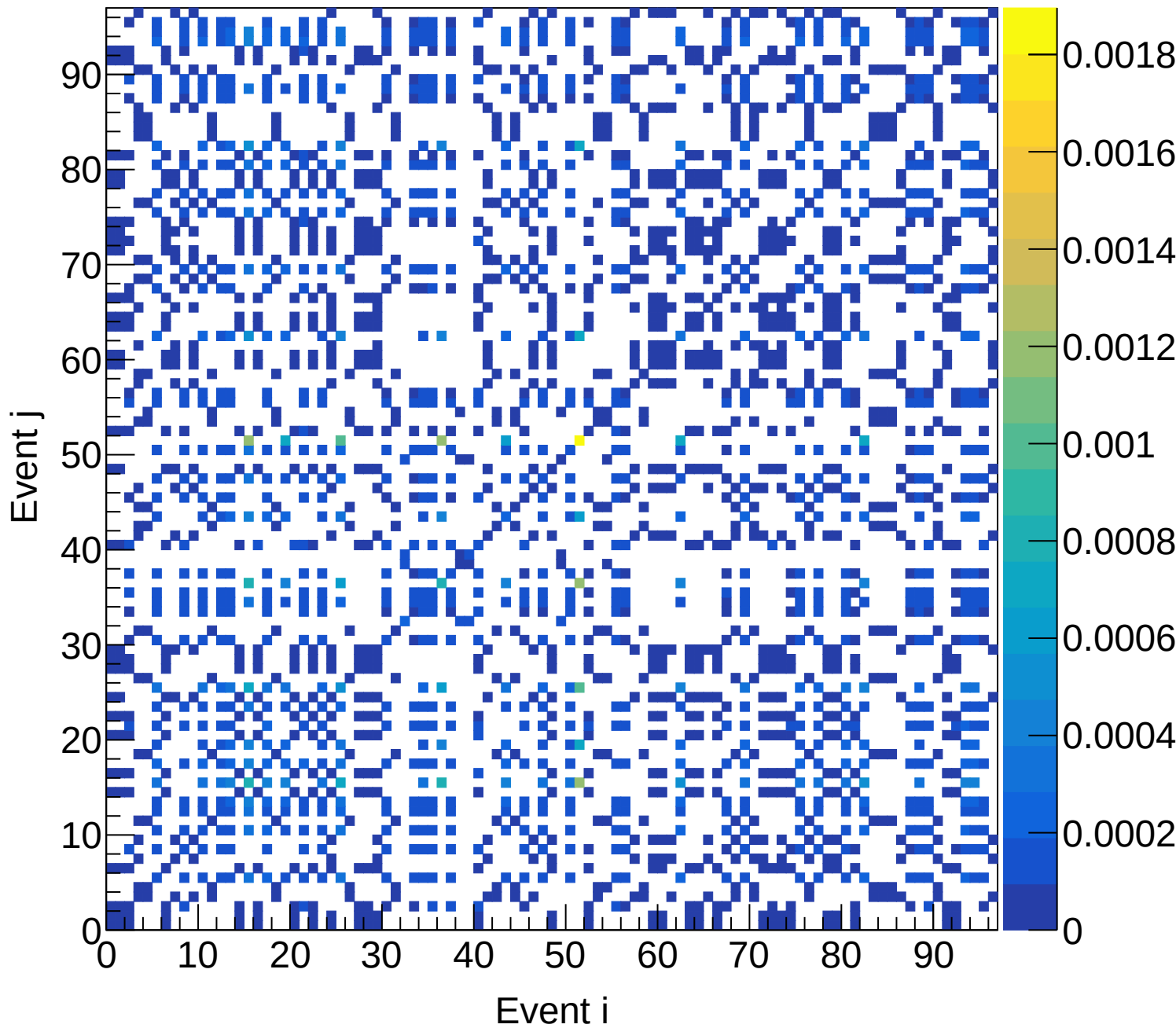
LD2 (total) Covariance | M: [4.5, 4.8) xF: [0.10, 0.15)
