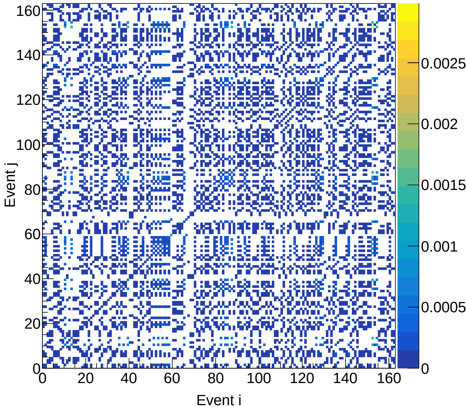
LD2 (total) Covariance | M: [4.8, 5.1) xF: [0.10, 0.15)
