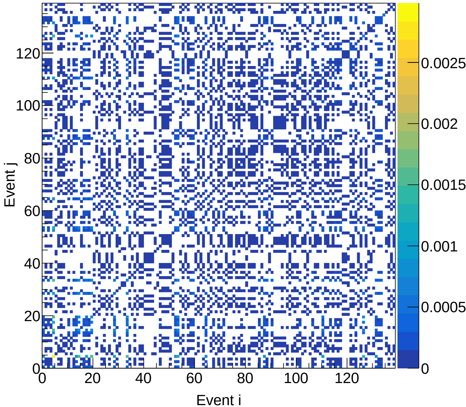
LD2 (total) Covariance | M: [5.1, 5.4) xF: [0.10, 0.15)
