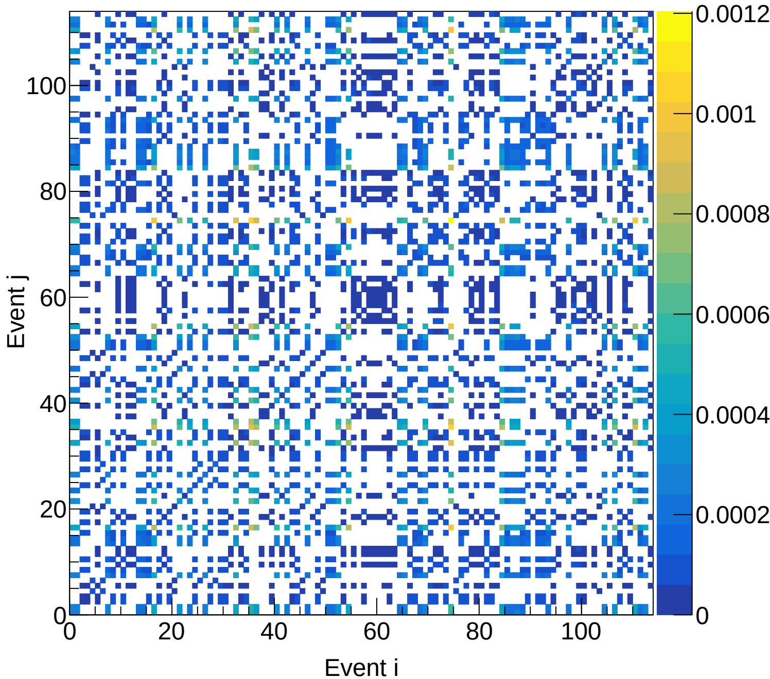
LD2 (total) Covariance | M: [5.4, 5.7) xF: [0.10, 0.15)
