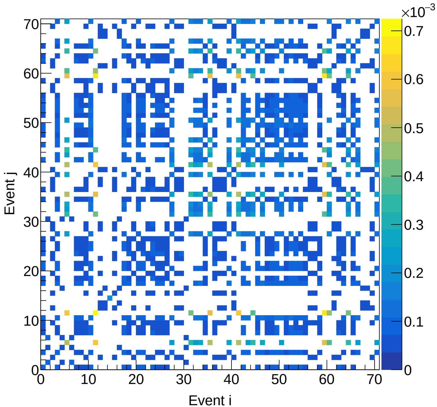
LD2 (total) Covariance | M: [5.7, 6.0] xF: [0.10, 0.15)
