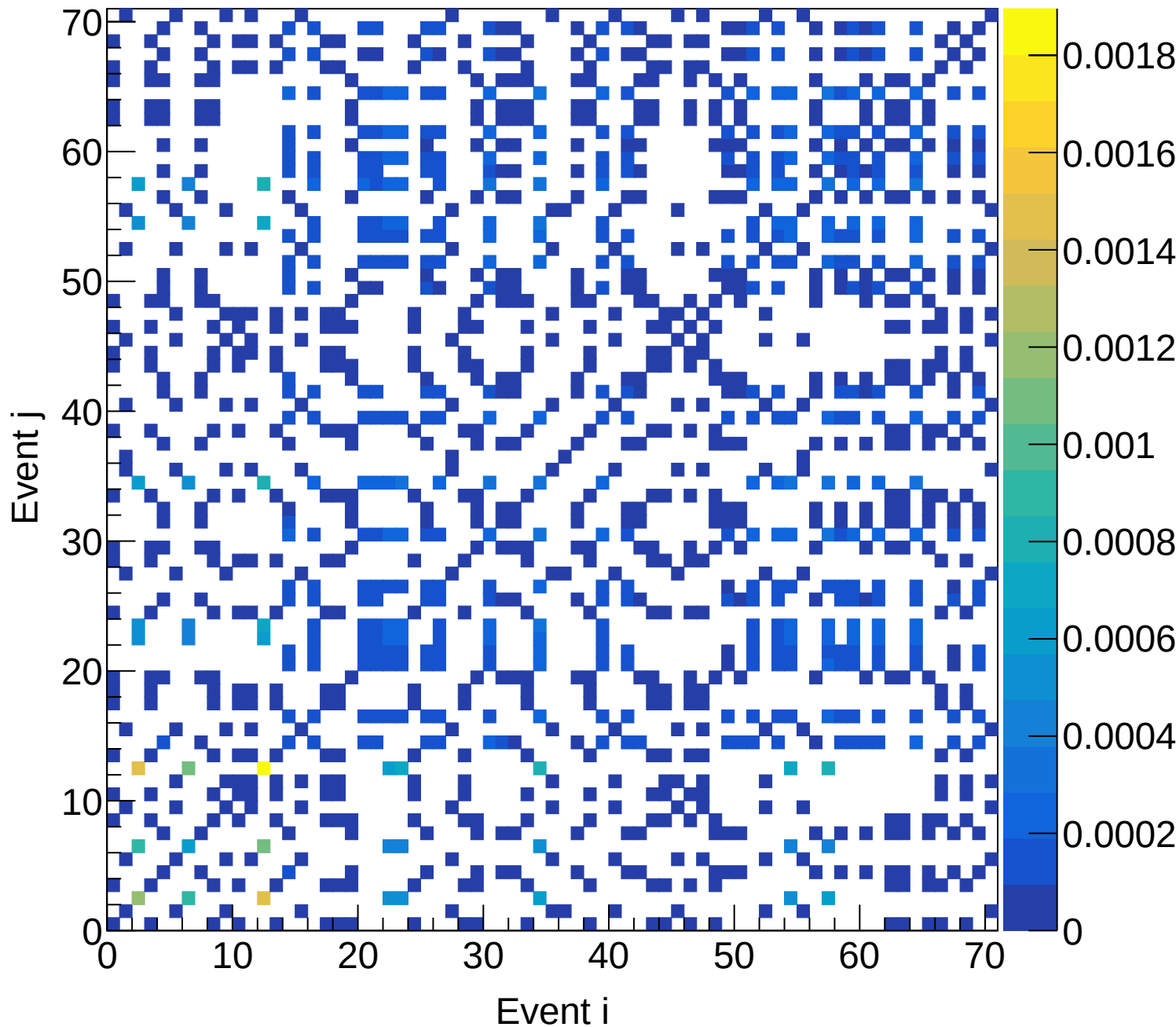
LD2 (total) Covariance | M: [4.2, 4.5) xF: [0.15, 0.20)
