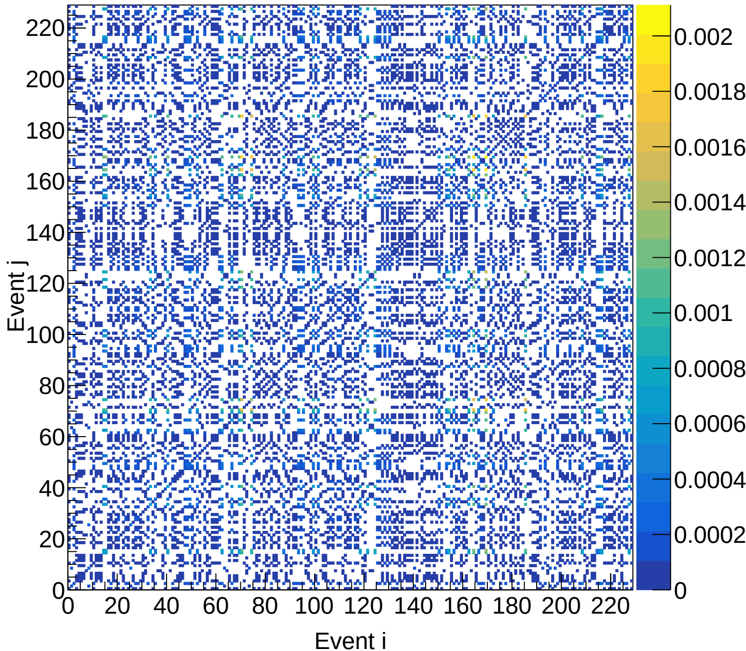
LD2 (total) Covariance | M: [4.8, 5.1) xF: [0.15, 0.20)
