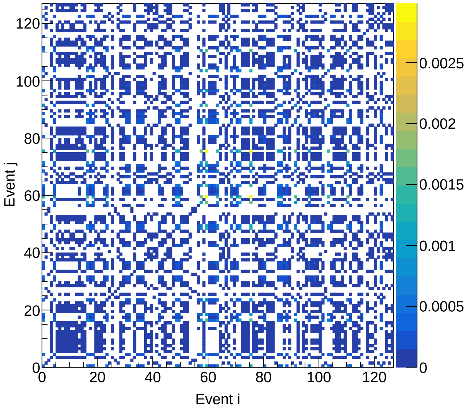
LD2 (total) Covariance | M: [5.4, 5.7) xF: [0.15, 0.20)
