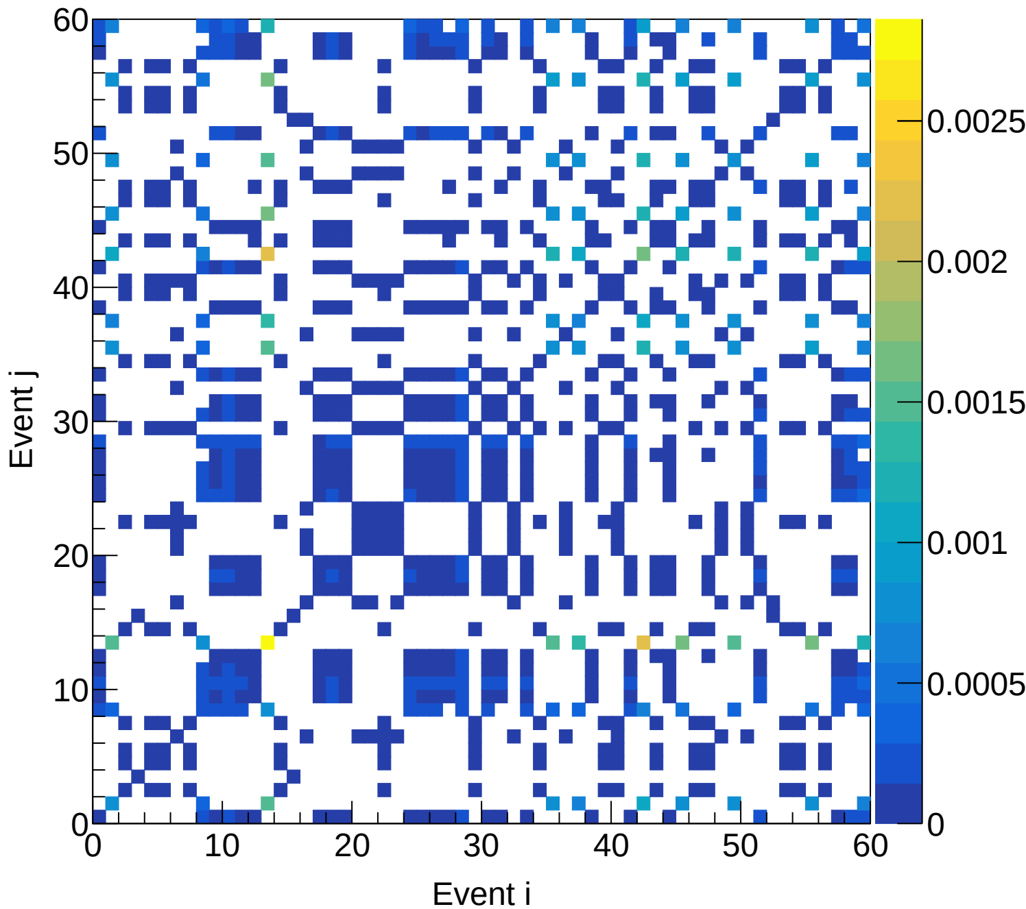
LD2 (total) Covariance | M: [6.0, 6.3) xF: [0.15, 0.20)
