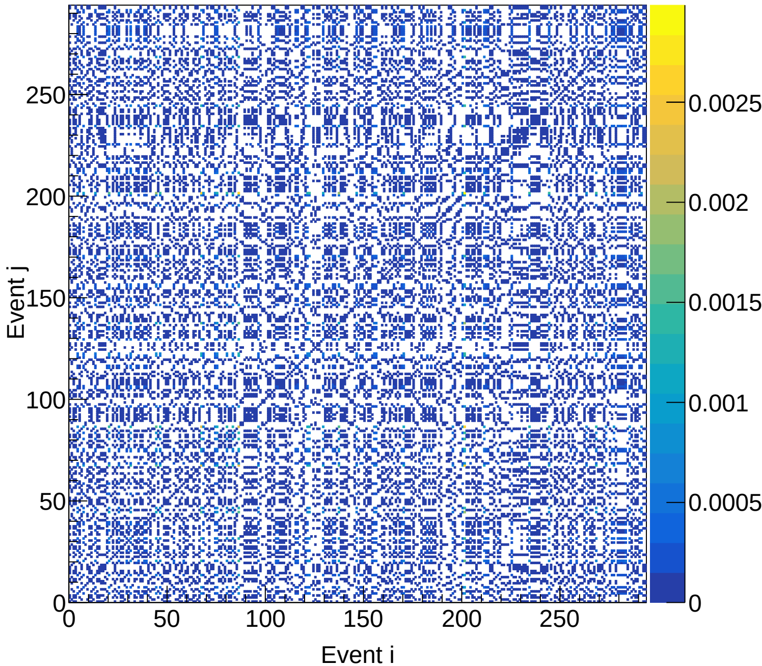
LD2 (total) Covariance | M: [4.5, 4.8) xF: [0.20, 0.25)
