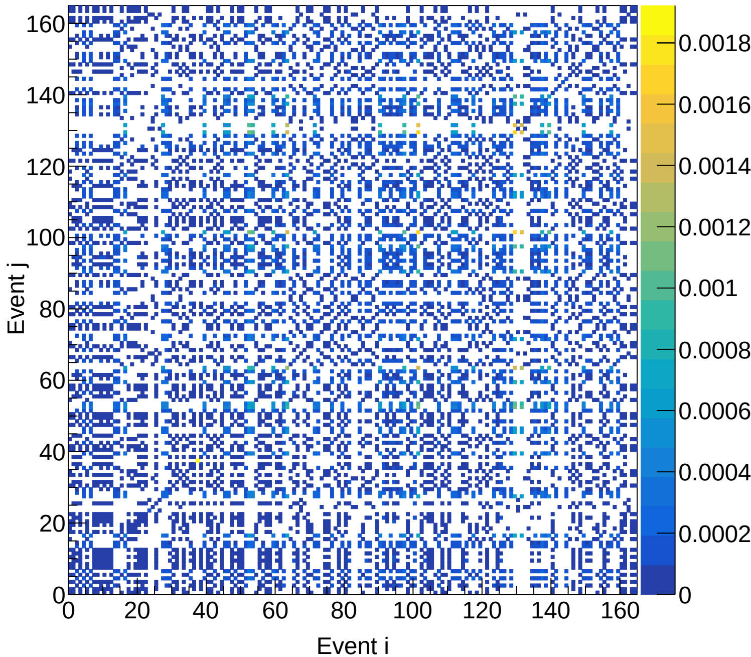
LD2 (total) Covariance | M: [5.4, 5.7) xF: [0.20, 0.25)
