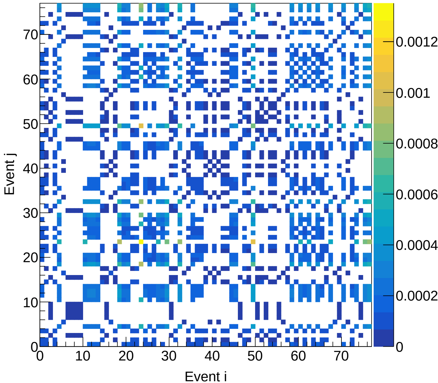
LD2 (total) Covariance | M: [6.0, 6.3) xF: [0.20, 0.25)
