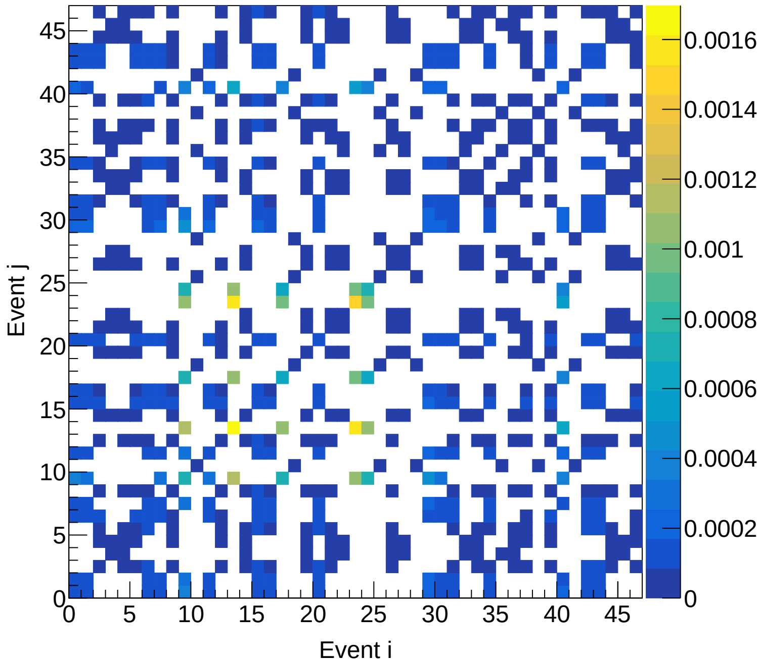
LD2 (total) Covariance | M: [6.3, 6.6] xF: [0.20, 0.25)
