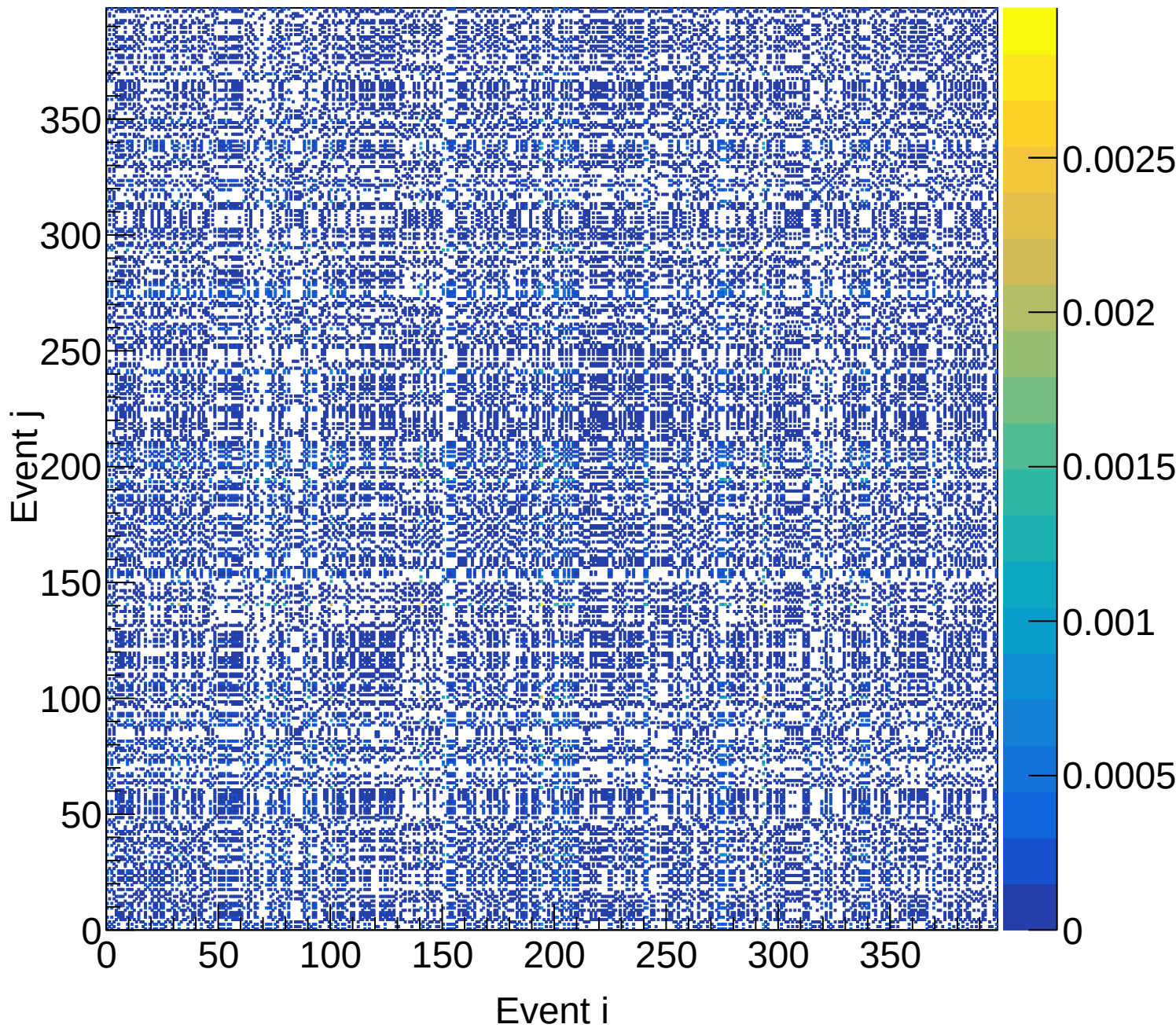
LD2 (total) Covariance | M: [4.2, 4.5) xF: [0.25, 0.30)
