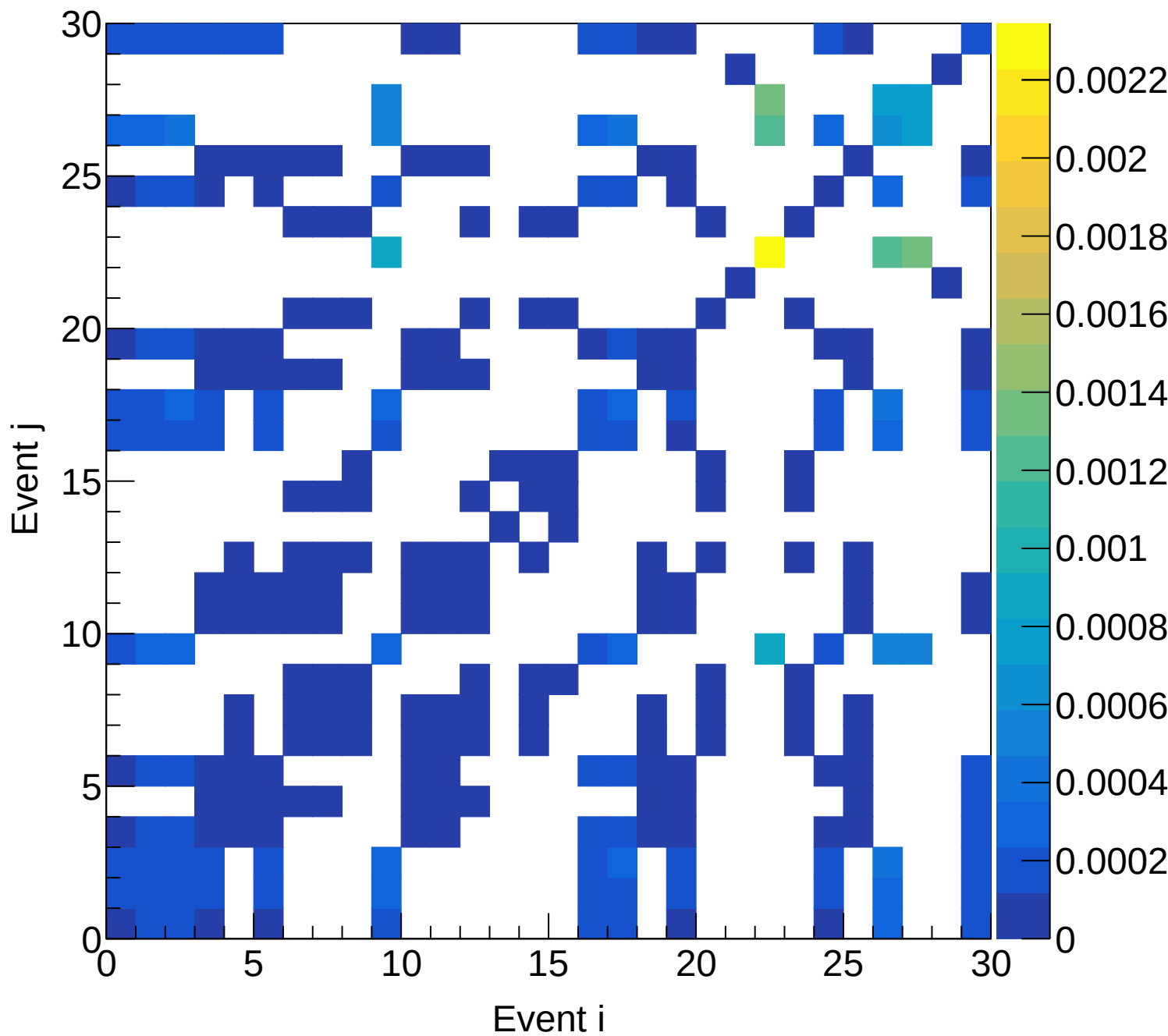
LD2 (total) Covariance | M: [6.9, 7.5] xF: [0.25, 0.30)
