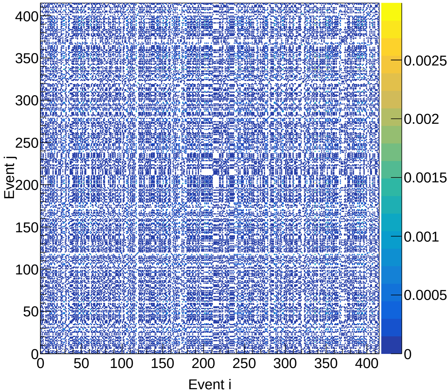
LD2 (total) Covariance | M: [4.5, 4.8) xF: [0.25, 0.30)
