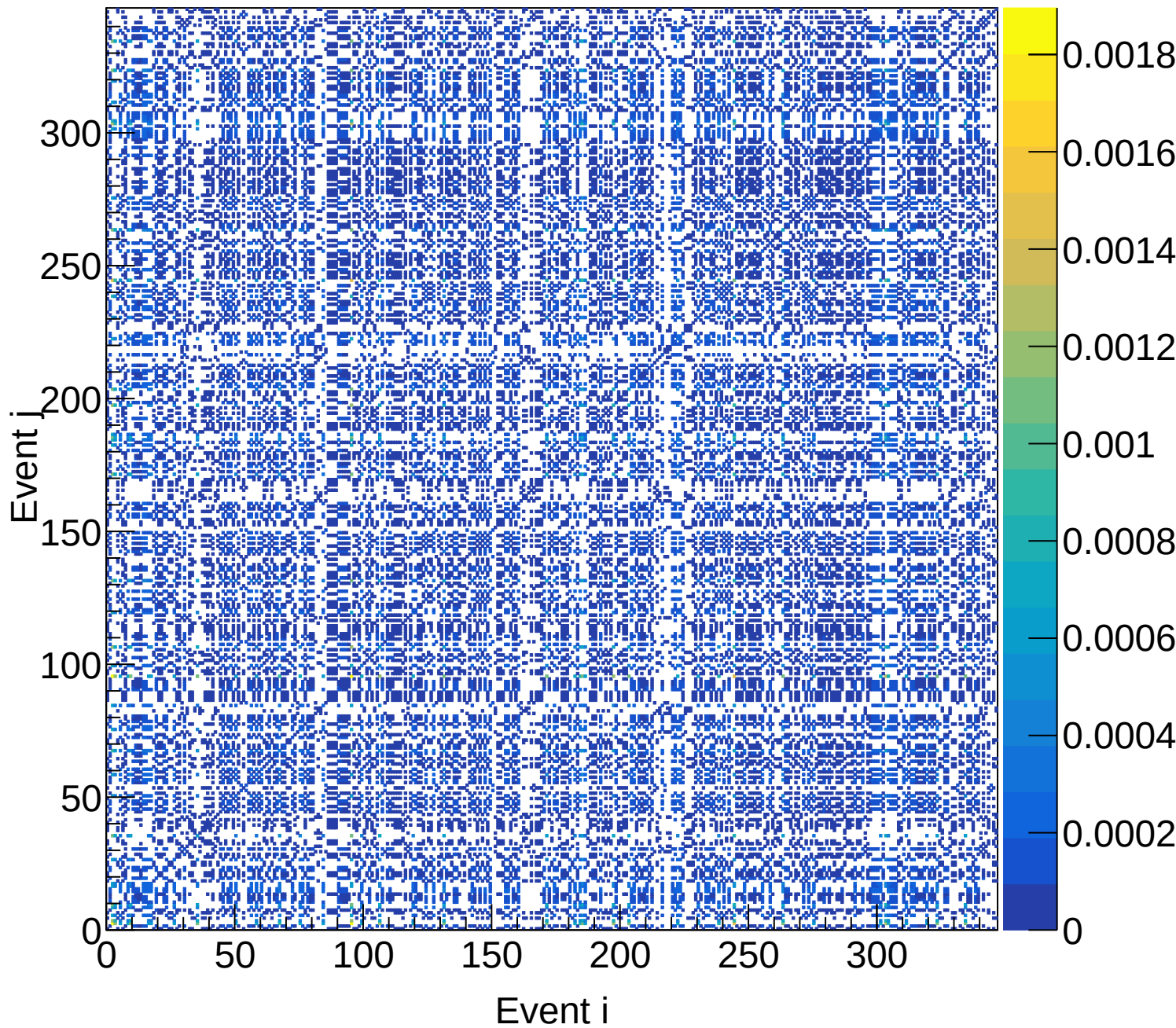
LD2 (total) Covariance | M: [4.8, 5.1) xF: [0.25, 0.30)
