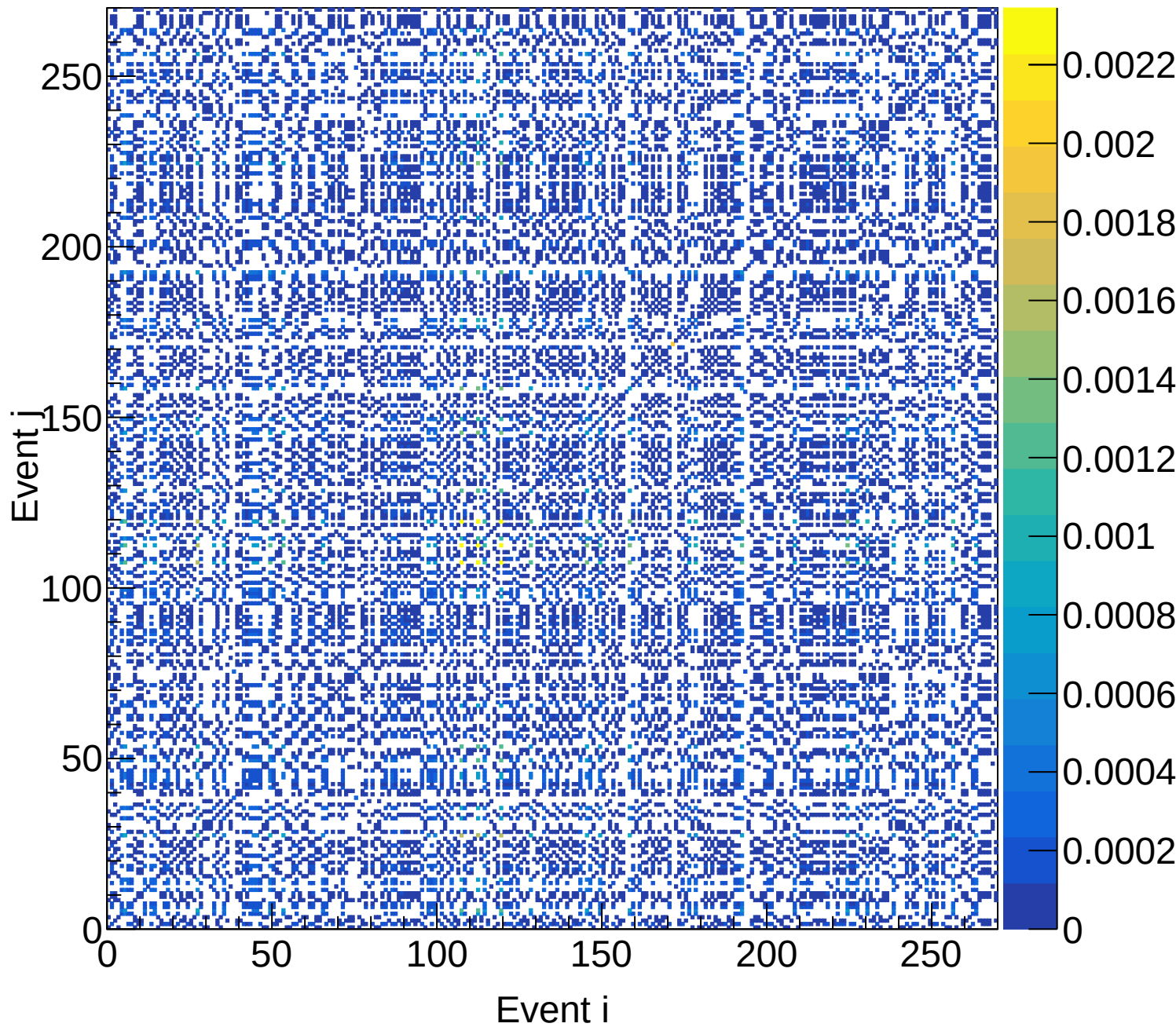
LD2 (total) Covariance | M: [5.1, 5.4) xF: [0.25, 0.30)
