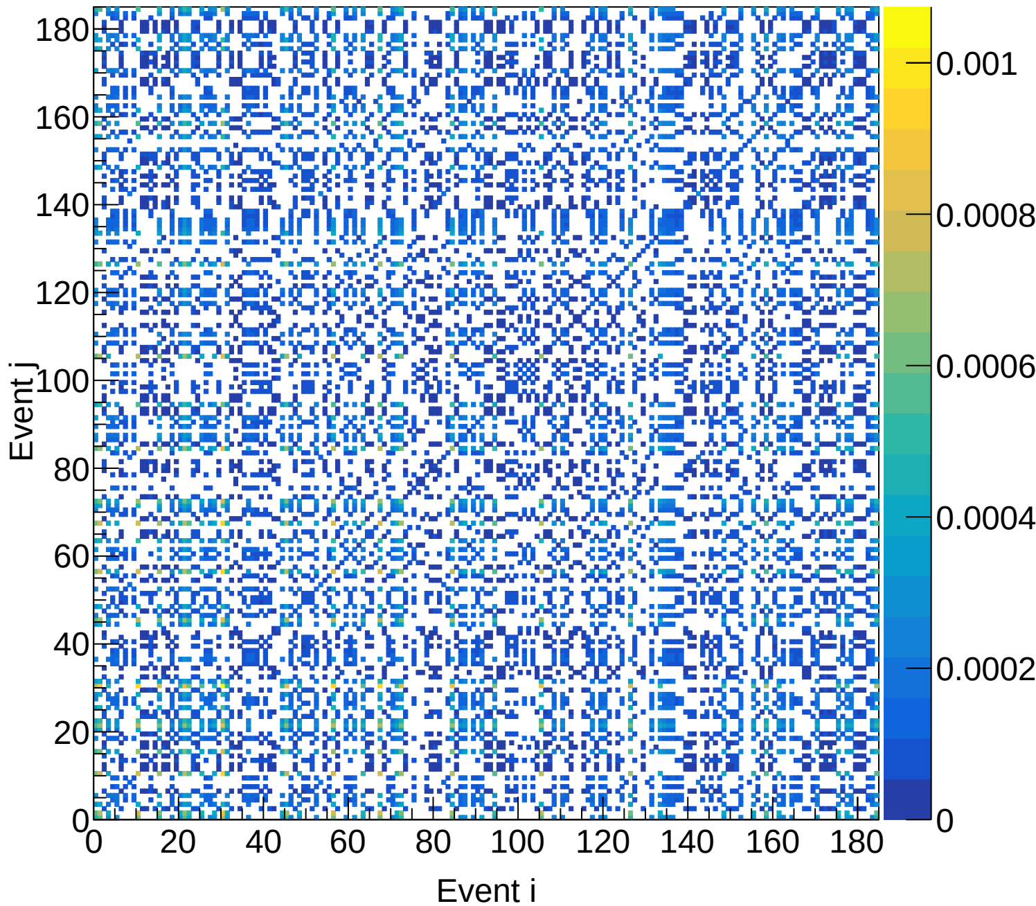
LD2 (total) Covariance | M: [5.4, 5.7) xF: [0.25, 0.30)
