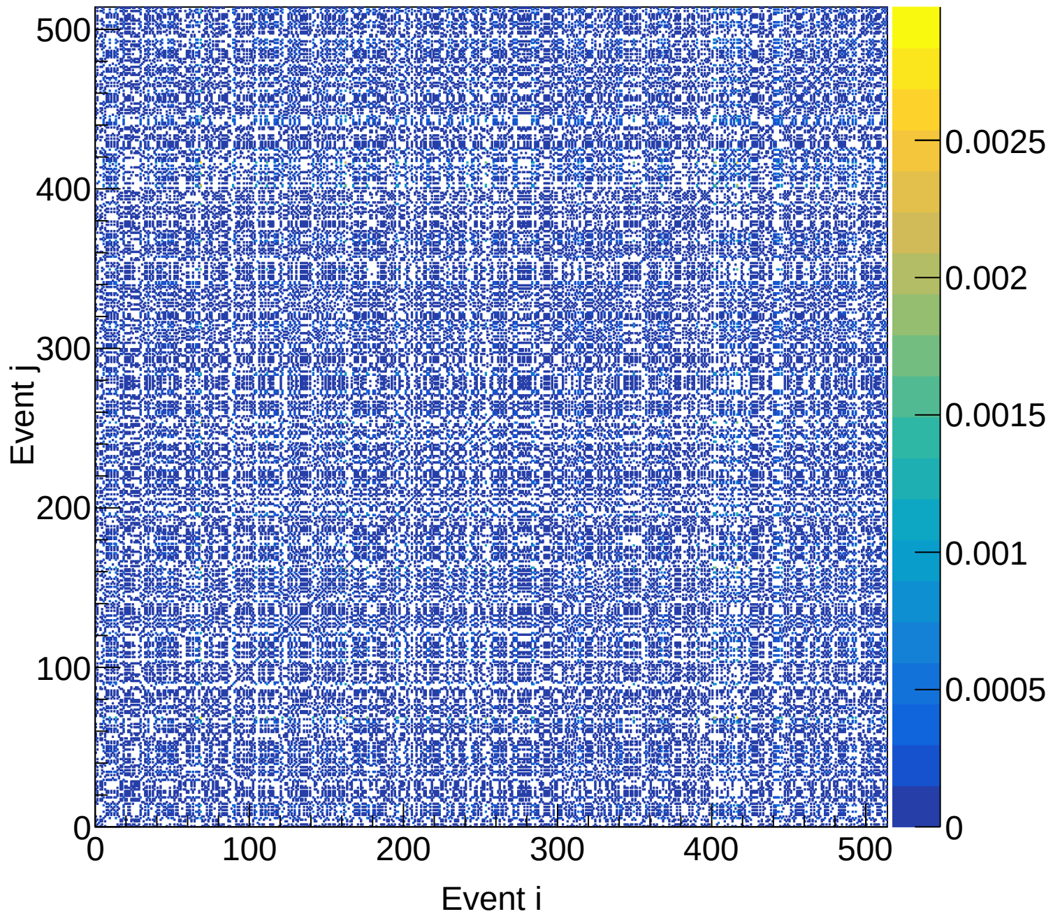
LD2 (total) Covariance | M: [4.5, 4.8) xF: [0.30, 0.35)
