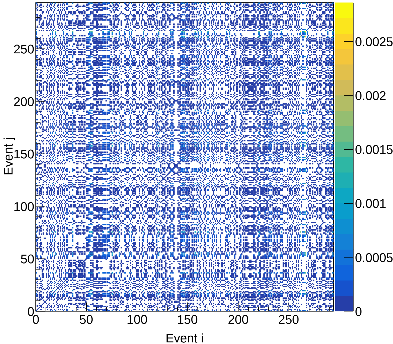
LD2 (total) Covariance | M: [5.1, 5.4) xF: [0.30, 0.35)
