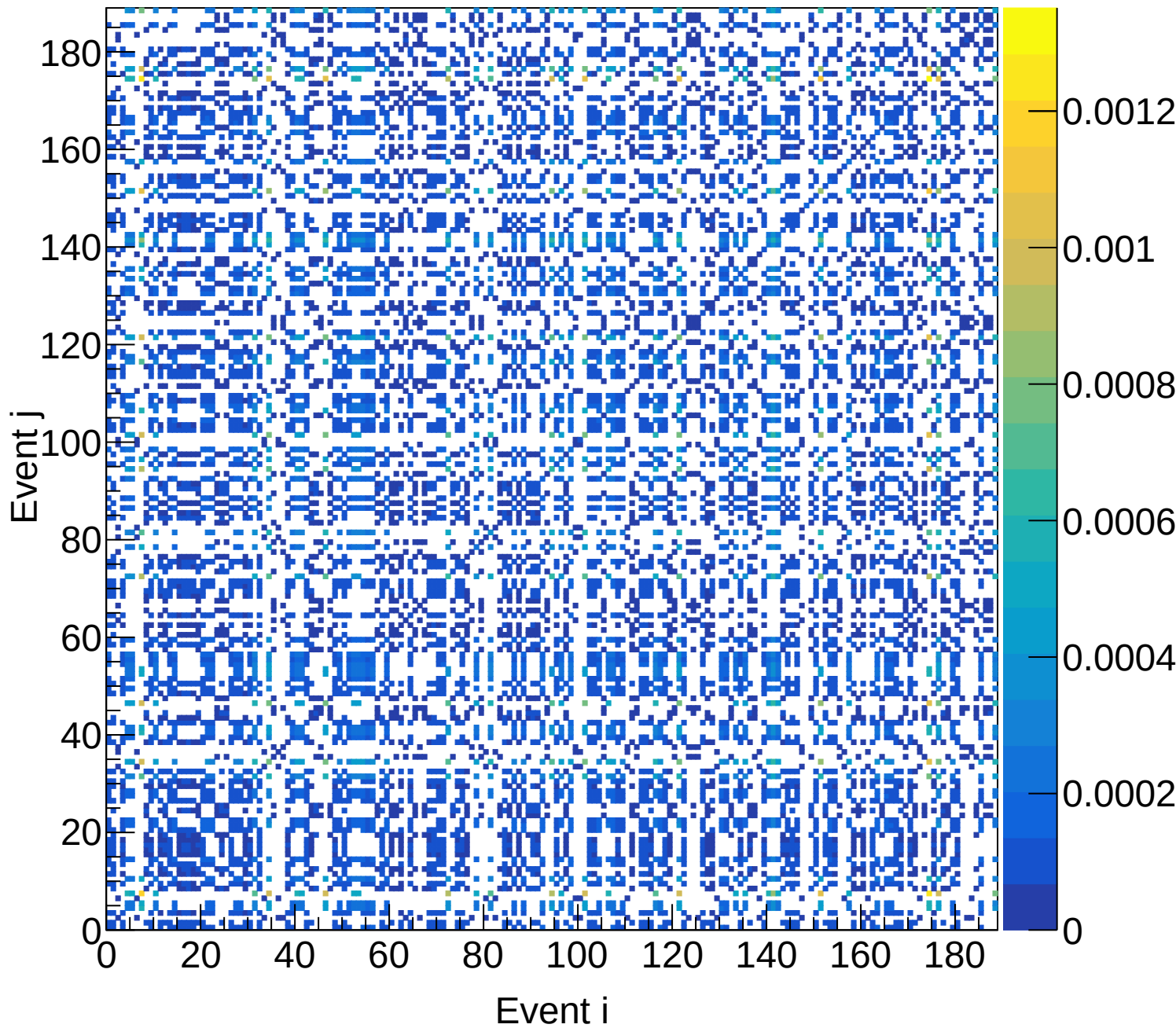
LD2 (total) Covariance | M: [5.4, 5.7) xF: [0.30, 0.35)
