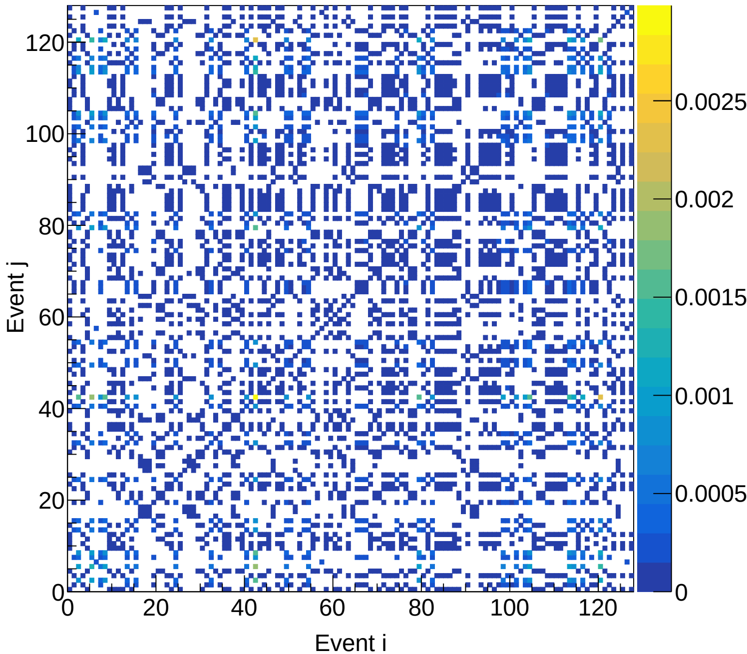
LD2 (total) Covariance | M: [5.7, 6.0) xF: [0.30, 0.35)
