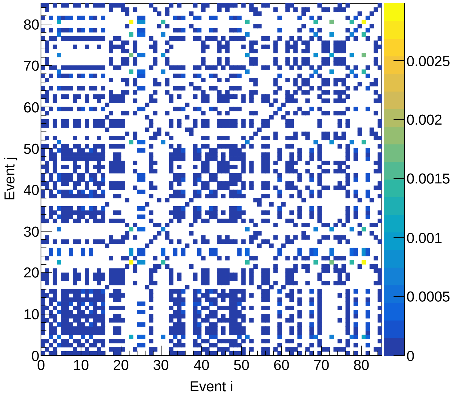
LD2 (total) Covariance | M: [6.0, 6.3] xF: [0.30, 0.35]
