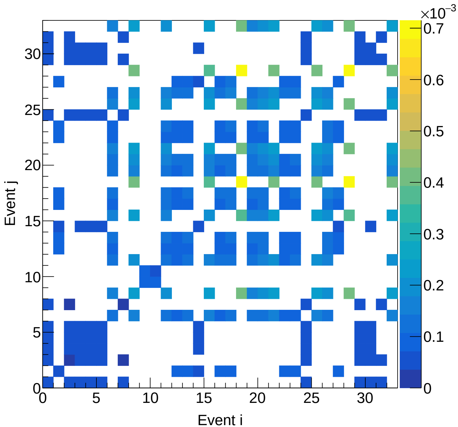
LD2 (total) Covariance | M: [6.6, 6.9) xF: [0.30, 0.35)
