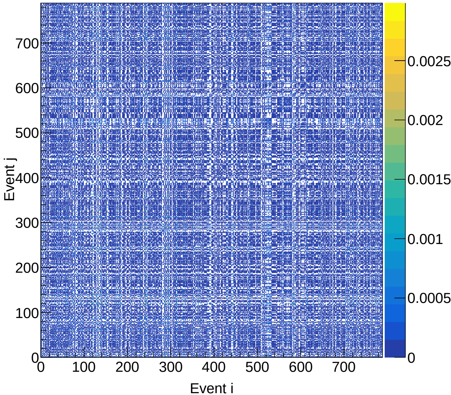
LD2 (total) Covariance | M: [3.9, 4.2) xF: [0.35, 0.40)
