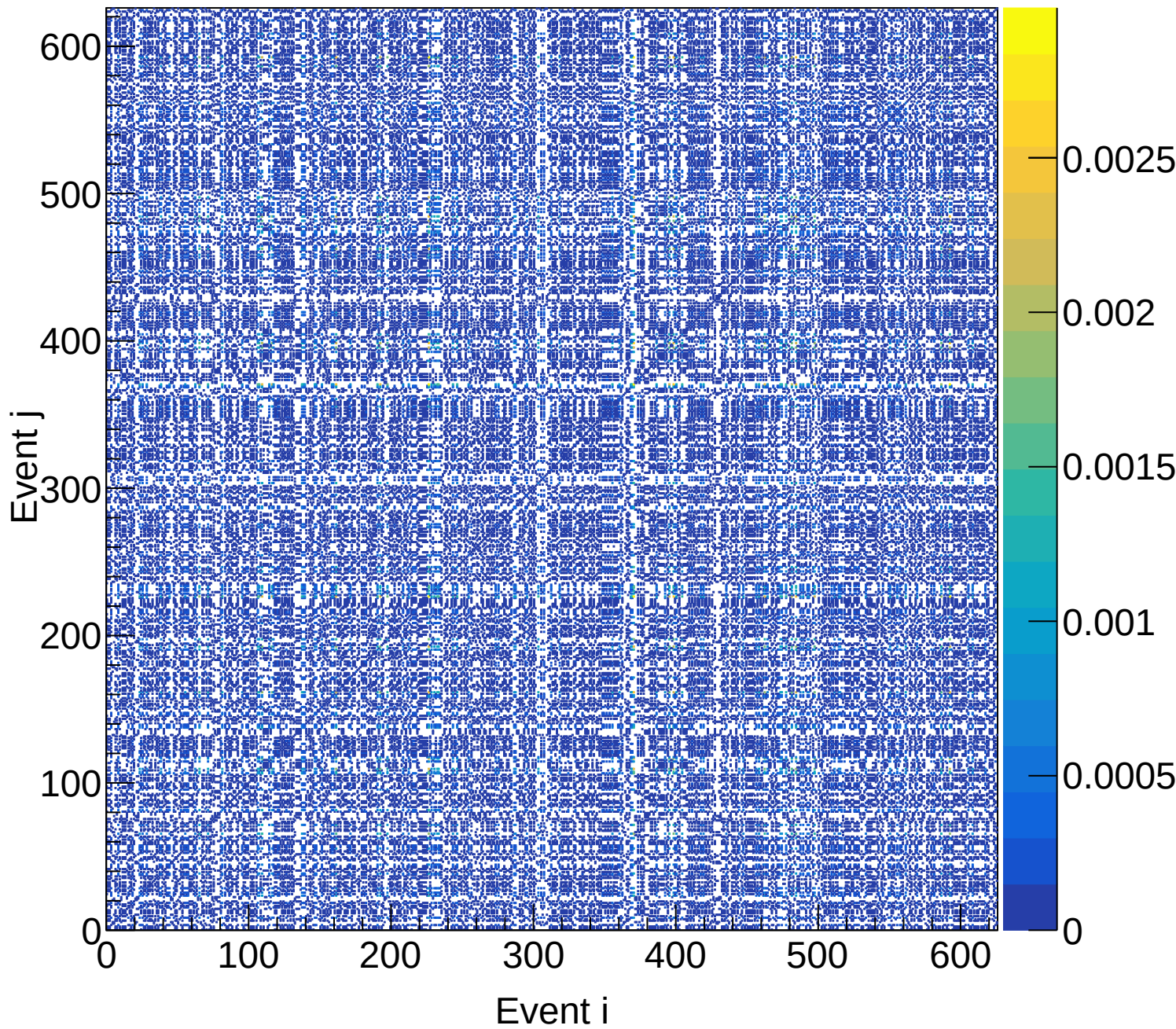
LD2 (total) Covariance | M: [4.2, 4.5) xF: [0.35, 0.40)
