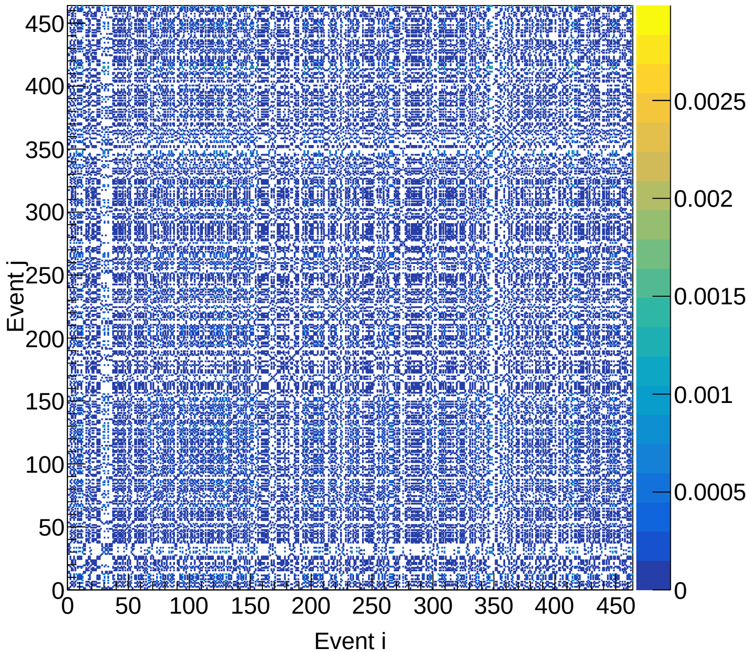
LD2 (total) Covariance | M: [4.8, 5.1) xF: [0.35, 0.40)
