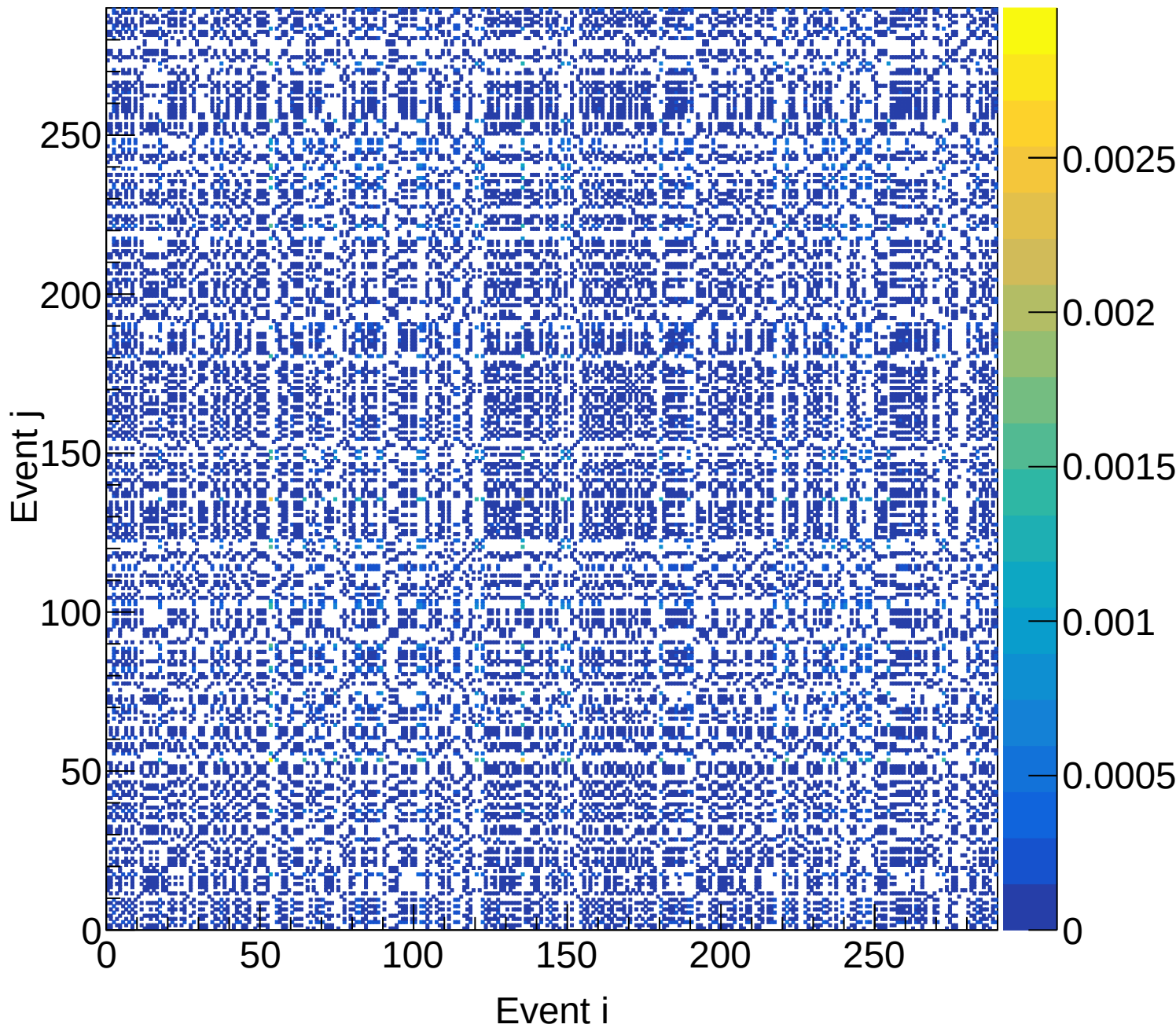
LD2 (total) Covariance | M: [5.1, 5.4) xF: [0.35, 0.40)
