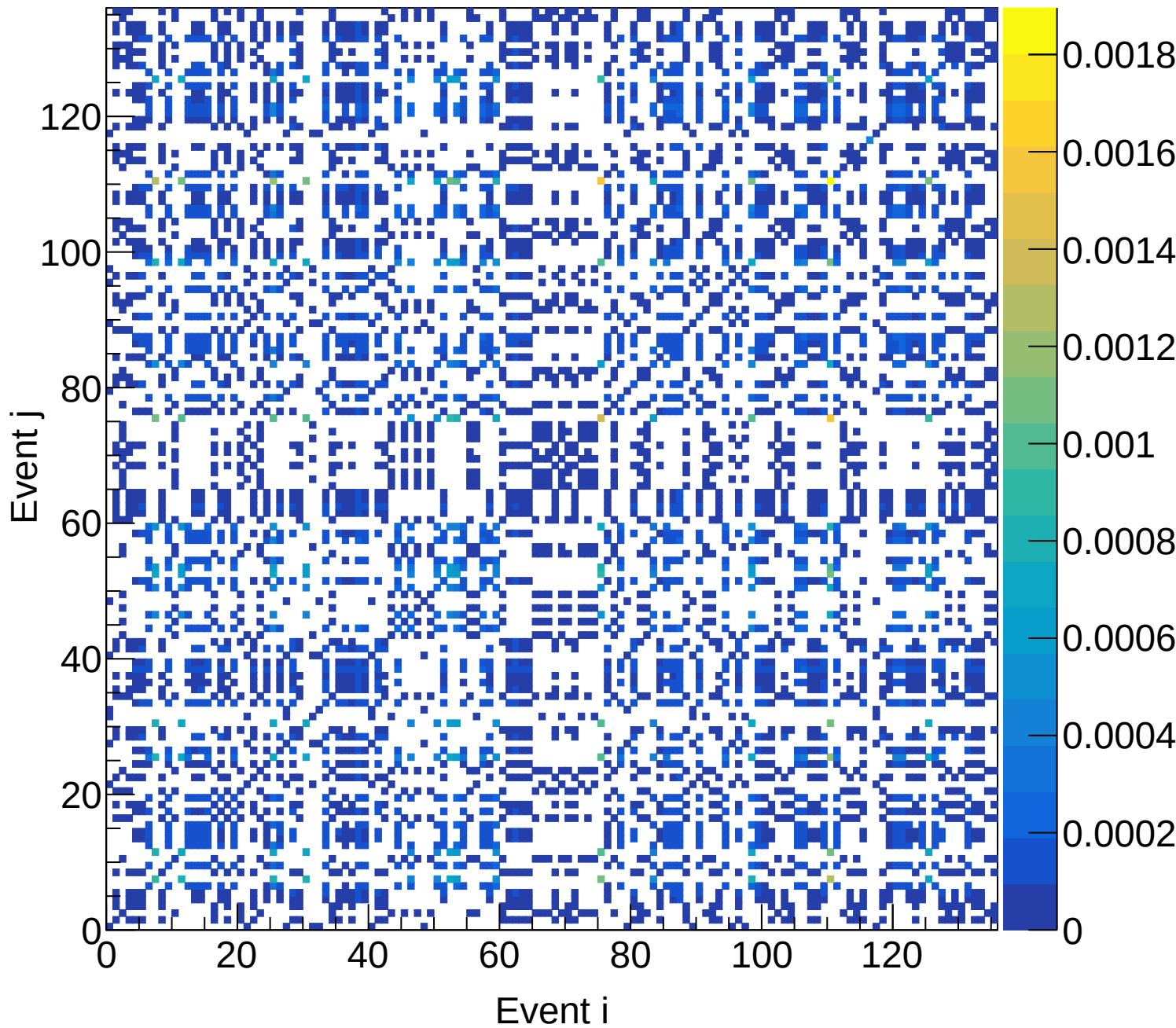
LD2 (total) Covariance | M: [5.7, 6.0) xF: [0.35, 0.40)
