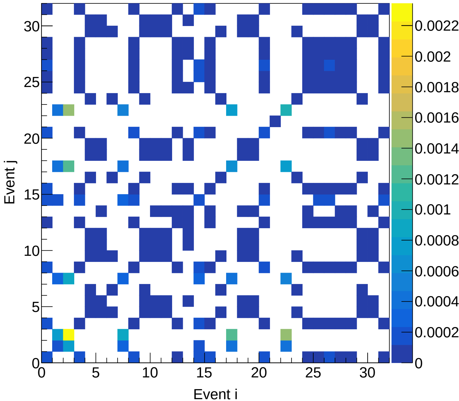
LD2 (total) Covariance | M: [6.6, 6.9) xF: [0.35, 0.40)
