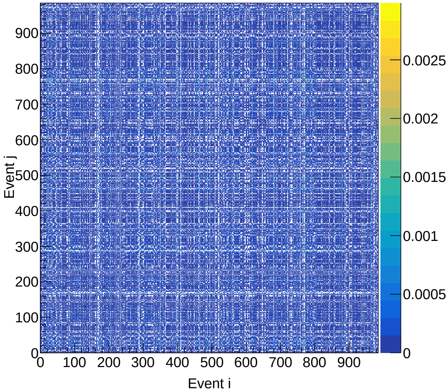
LD2 (total) Covariance | M: [3.9, 4.2) xF: [0.40, 0.45)
