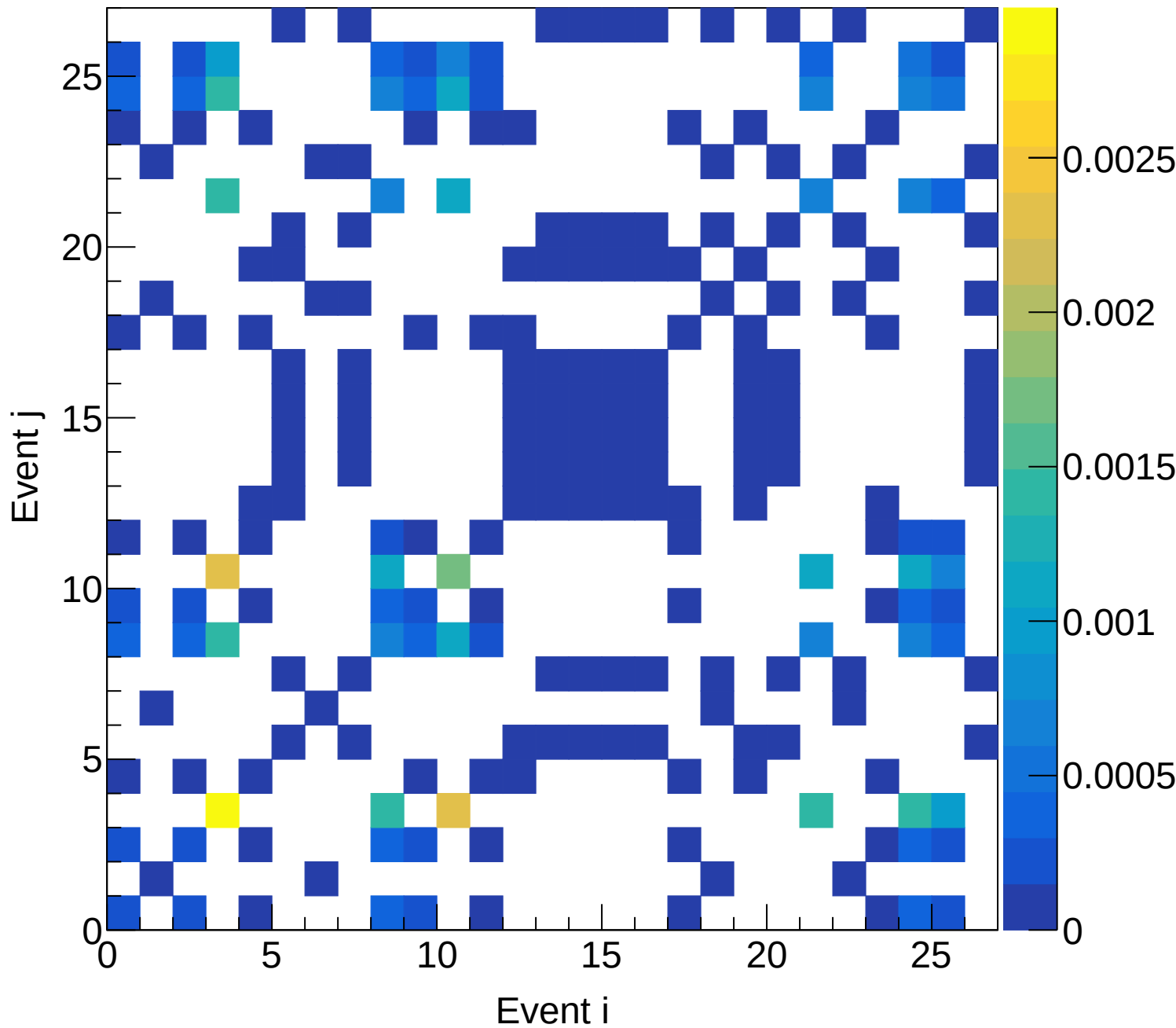
LD2 (total) Covariance | M: [6.9, 7.5) xF: [0.40, 0.45)
