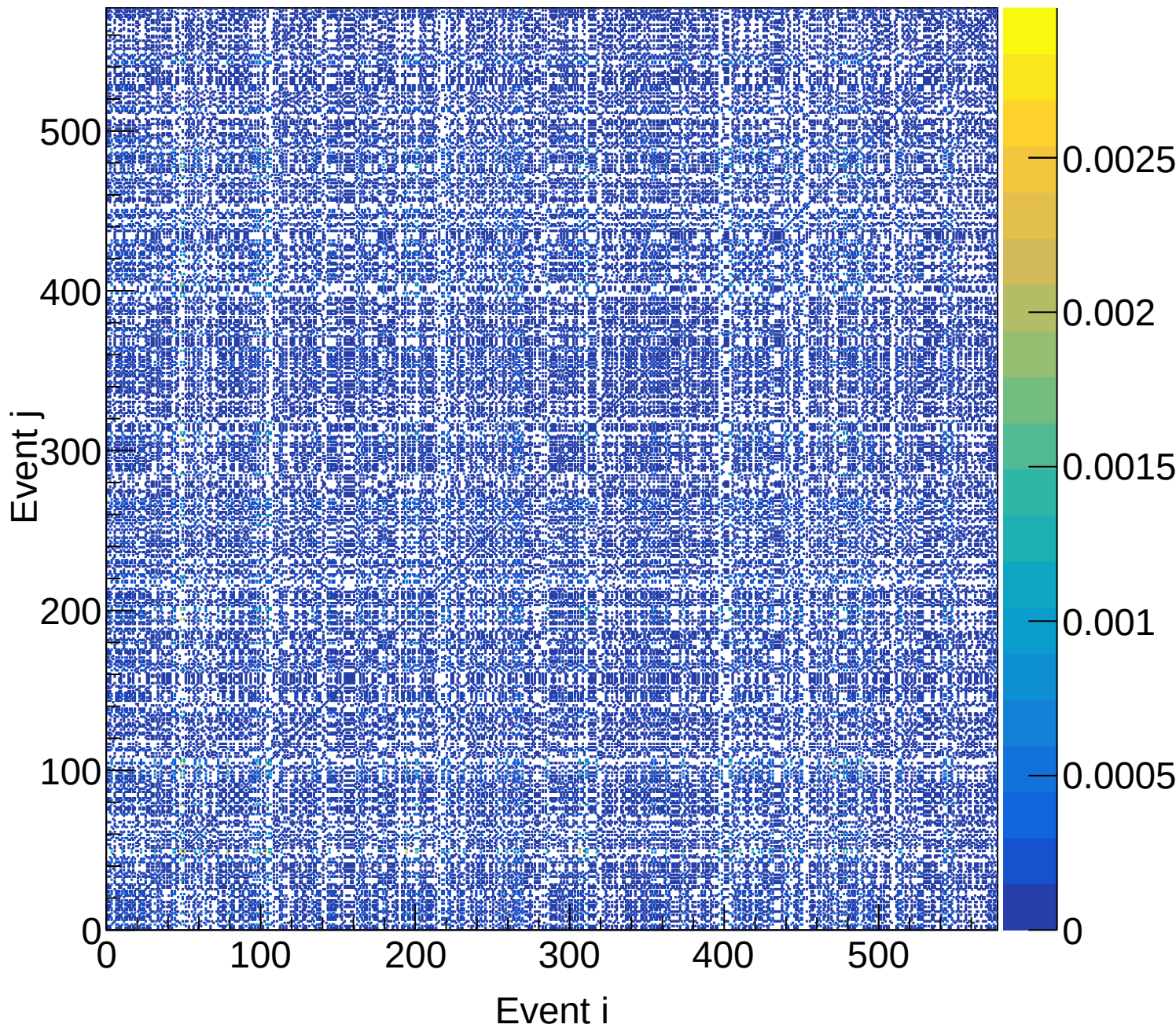
LD2 (total) Covariance | M: [4.5, 4.8) xF: [0.40, 0.45)
