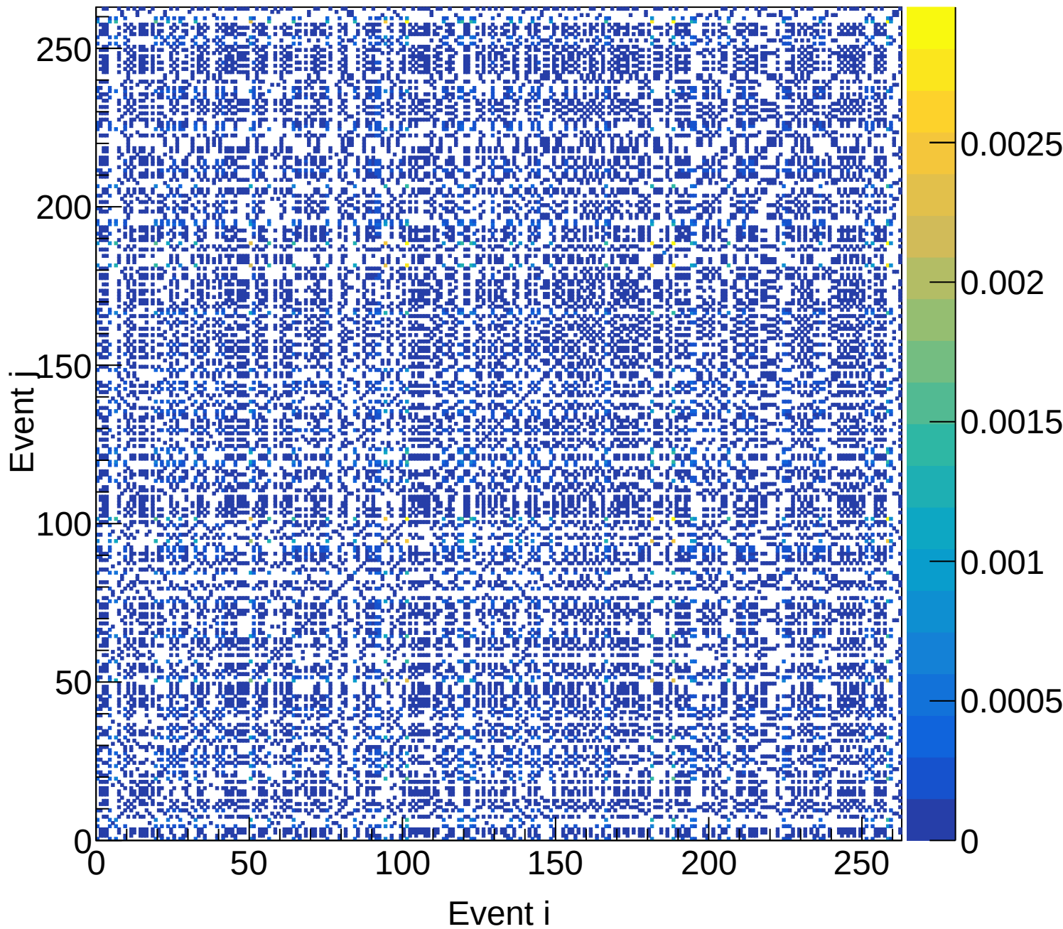
LD2 (total) Covariance | M: [5.1, 5.4) xF: [0.40, 0.45)
