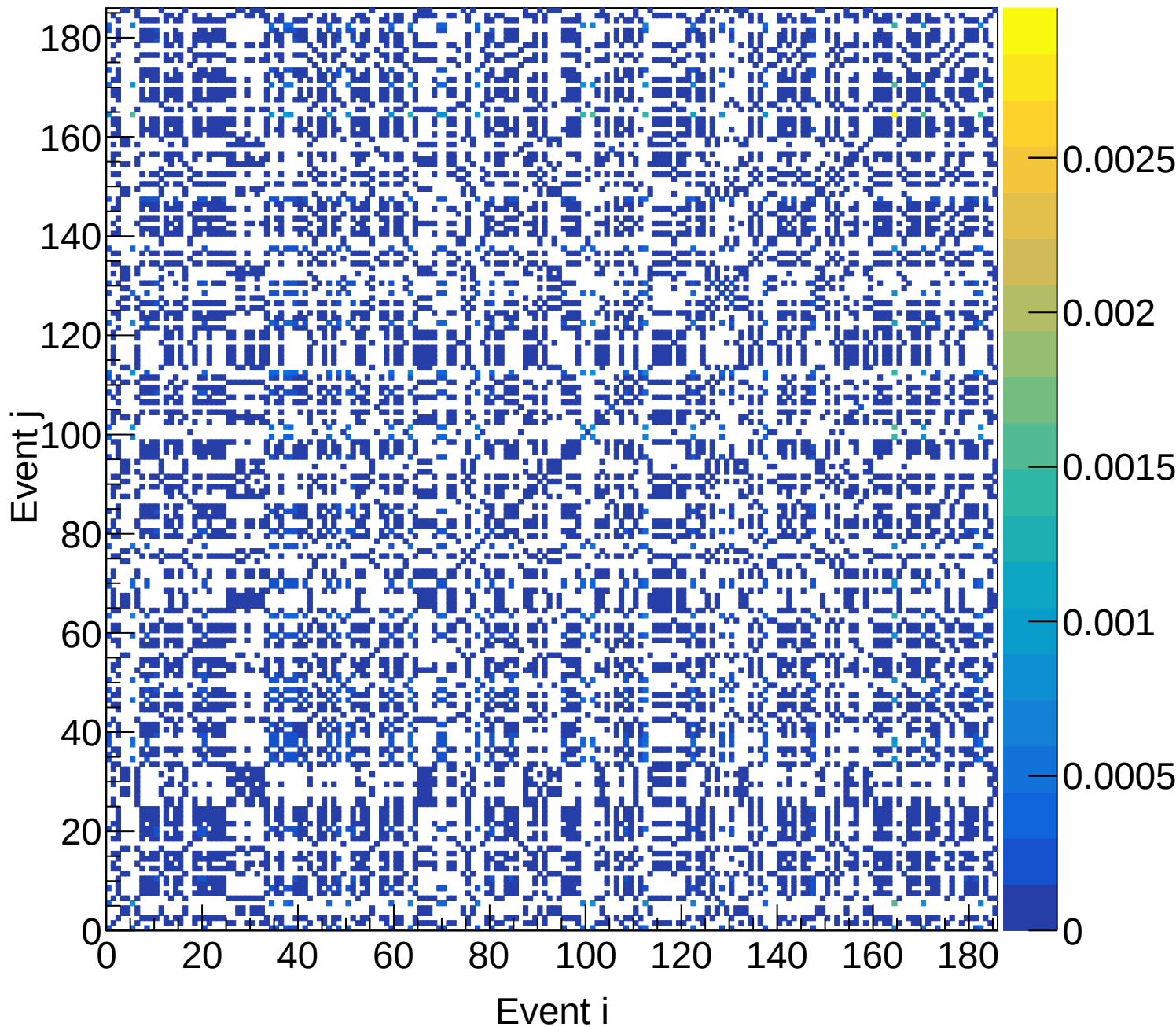
LD2 (total) Covariance | M: [5.4, 5.7) xF: [0.40, 0.45)
