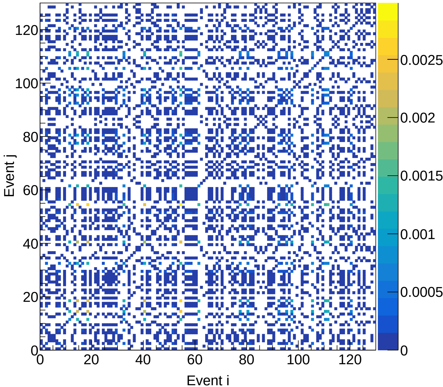
LD2 (total) Covariance | M: [5.7, 6.0] xF: [0.40, 0.45)
